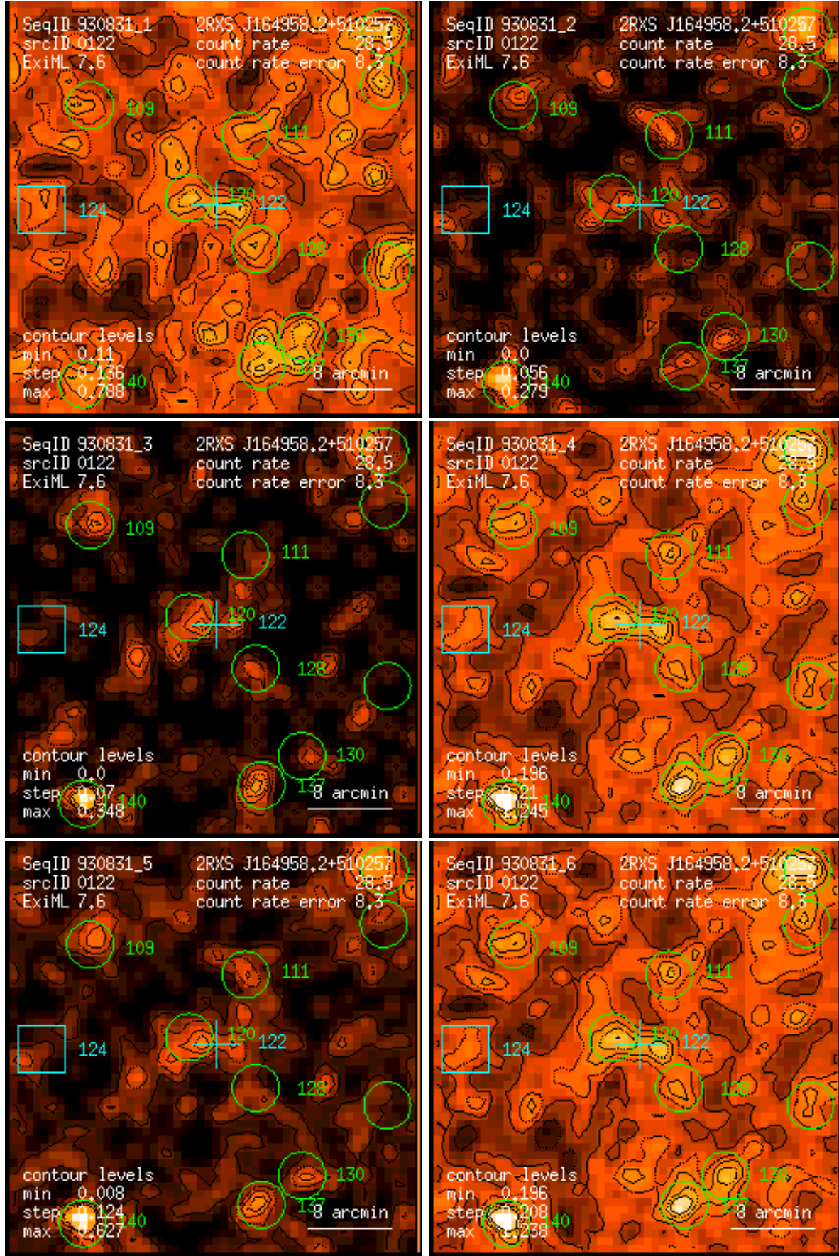
Figure 122: RASS 930831: detection 0122: band rate images, Gaussian filter: (1) PSPC channels 11 – 41, (2) 52 – 90, (3) 91 – 201, (4) 11 – 235, (5) 52 – 201, (6) 11 – 201. Broad band rates in counts/ks. Band rate contour levels in counts/ks/arcmin 2 .
