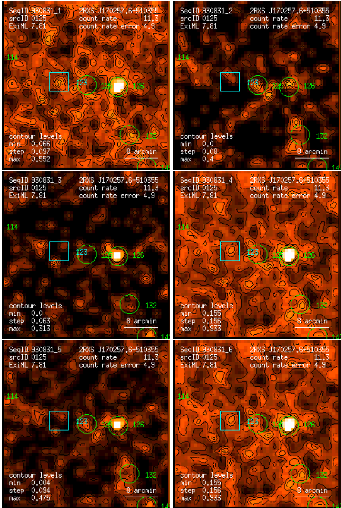
Figure 125: RASS 930831: detection 0125: band rate images, Gaussian filter: (1) PSPC channels 11 – 41, (2) 52 – 90, (3) 91 – 201, (4) 11 – 235, (5) 52 – 201, (6) 11 – 201. Broad band rates in counts/ks. Band rate contour levels in counts/ks/arcmin 2 .
