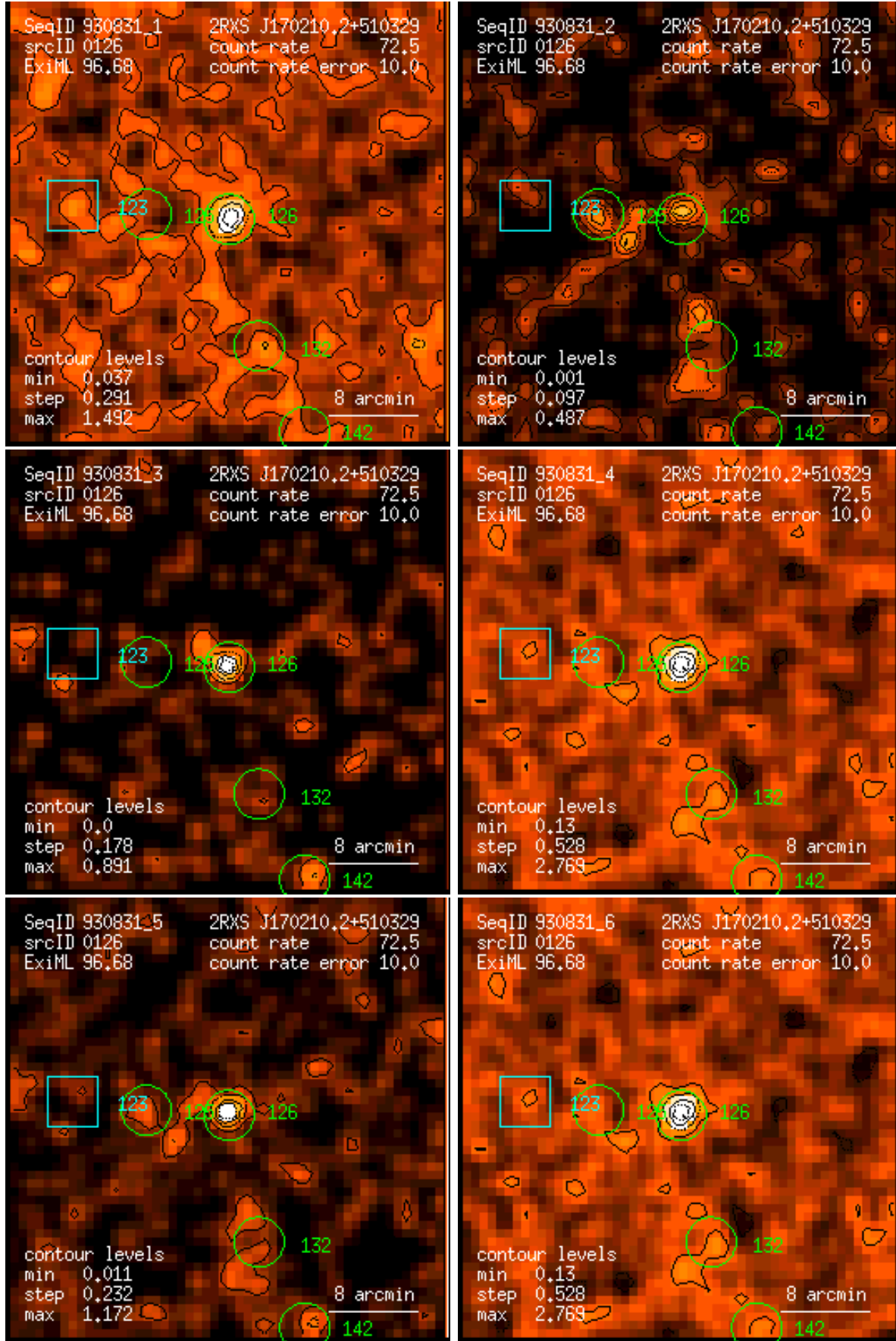
Figure 126: RASS 930831: detection 0126: band rate images, Gaussian filter: (1) PSPC channels 11 – 41, (2) 52 – 90, (3) 91 – 201, (4) 11 – 235, (5) 52 – 201, (6) 11 – 201. Broad band rates in counts/ks. Band rate contour levels in counts/ks/arcmin 2 .
