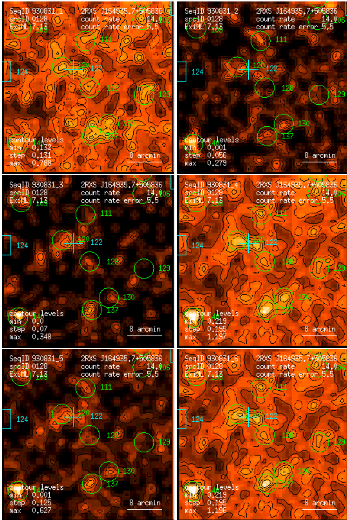
Figure 128: RASS 930831: detection 0128: band rate images, Gaussian filter: (1) PSPC channels 11 – 41, (2) 52 – 90, (3) 91 – 201, (4) 11 – 235, (5) 52 – 201, (6) 11 – 201. Broad band rates in counts/ks. Band rate contour levels in counts/ks/arcmin 2 .
