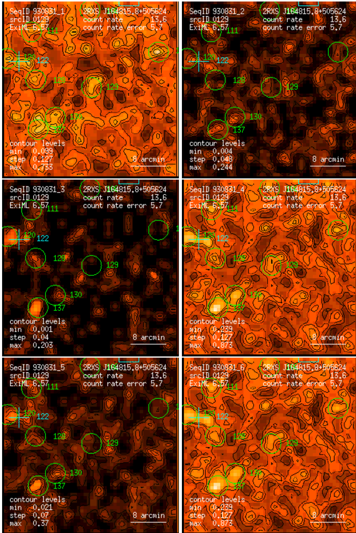
Figure 129: RASS 930831: detection 0129: band rate images, Gaussian filter: (1) PSPC channels 11 – 41, (2) 52 – 90, (3) 91 – 201, (4) 11 – 235, (5) 52 – 201, (6) 11 – 201. Broad band rates in counts/ks. Band rate contour levels in counts/ks/arcmin 2 .
