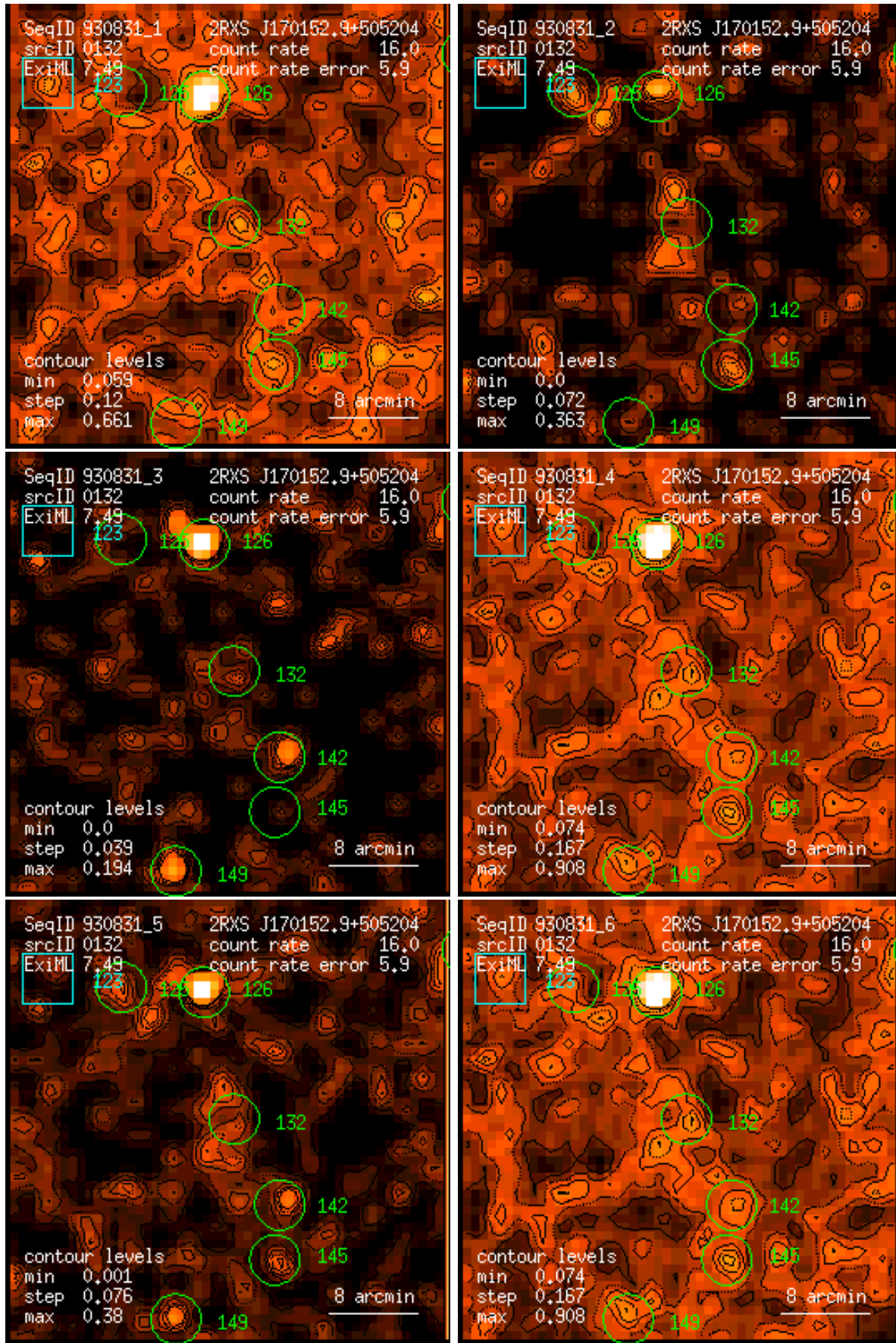
Figure 132: RASS 930831: detection 0132: band rate images, Gaussian filter: (1) PSPC channels 11 – 41, (2) 52 – 90, (3) 91 – 201, (4) 11 – 235, (5) 52 – 201, (6) 11 – 201. Broad band rates in counts/ks. Band rate contour levels in counts/ks/arcmin 2 .
