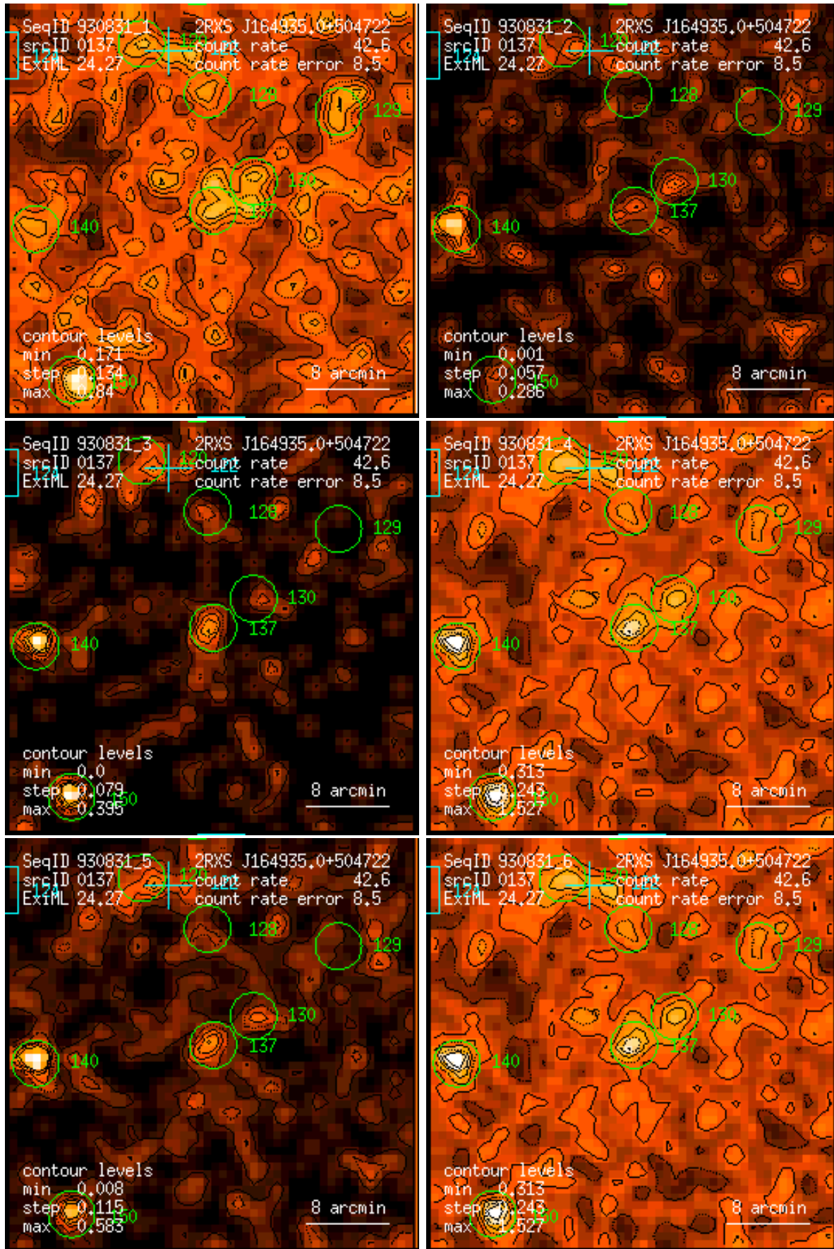
Figure 137: RASS 930831: detection 0137: band rate images, Gaussian filter: (1) PSPC channels 11 – 41, (2) 52 – 90, (3) 91 – 201, (4) 11 – 235, (5) 52 – 201, (6) 11 – 201. Broad band rates in counts/ks. Band rate contour levels in counts/ks/arcmin 2 .
