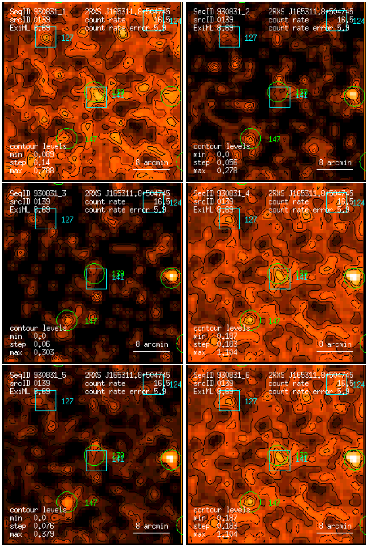
Figure 139: RASS 930831: detection 0139: band rate images, Gaussian filter: (1) PSPC channels 11 – 41, (2) 52 – 90, (3) 91 – 201, (4) 11 – 235, (5) 52 – 201, (6) 11 – 201. Broad band rates in counts/ks. Band rate contour levels in counts/ks/arcmin 2 .
