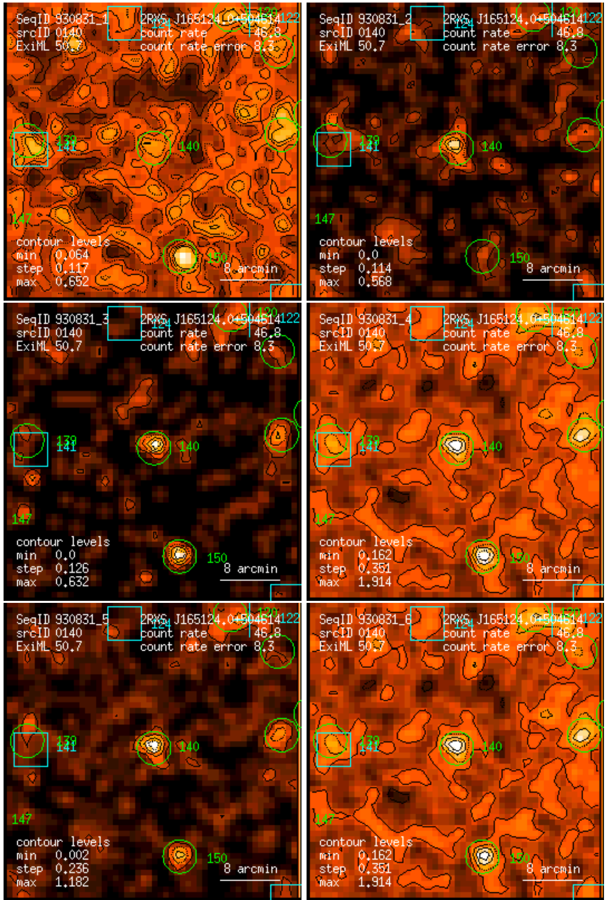
Figure 140: RASS 930831: detection 0140: band rate images, Gaussian filter: (1) PSPC channels 11 – 41, (2) 52 – 90, (3) 91 – 201, (4) 11 – 235, (5) 52 – 201, (6) 11 – 201. Broad band rates in counts/ks. Band rate contour levels in counts/ks/arcmin 2 .
