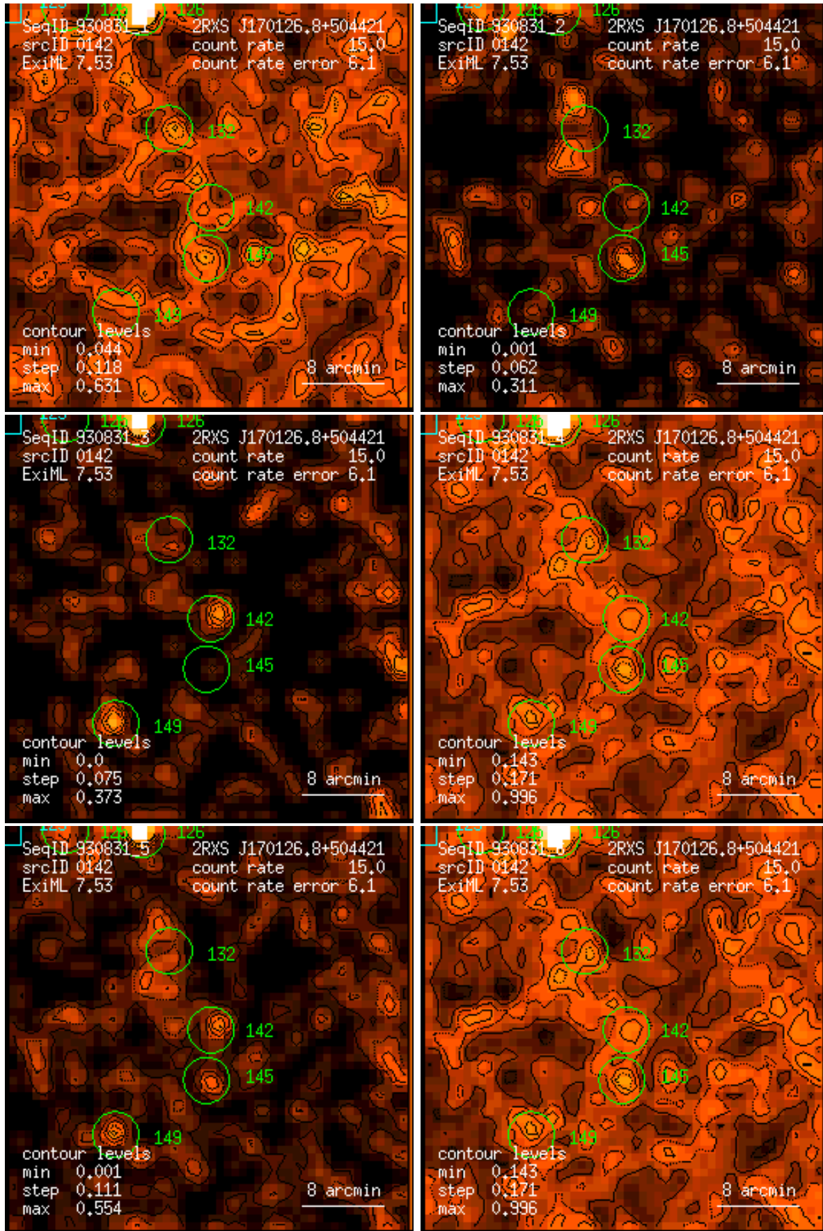
Figure 142: RASS 930831: detection 0142: band rate images, Gaussian filter: (1) PSPC channels 11 – 41, (2) 52 – 90, (3) 91 – 201, (4) 11 – 235, (5) 52 – 201, (6) 11 – 201. Broad band rates in counts/ks. Band rate contour levels in counts/ks/arcmin 2 .
