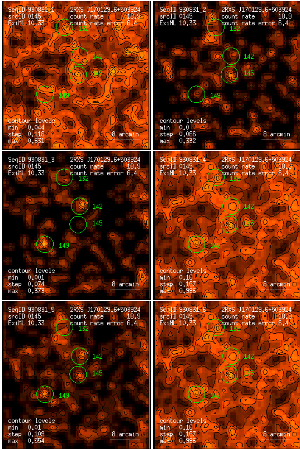
Figure 145: RASS 930831: detection 0145: band rate images, Gaussian filter: (1) PSPC channels 11 – 41, (2) 52 – 90, (3) 91 – 201, (4) 11 – 235, (5) 52 – 201, (6) 11 – 201. Broad band rates in counts/ks. Band rate contour levels in counts/ks/arcmin 2 .
