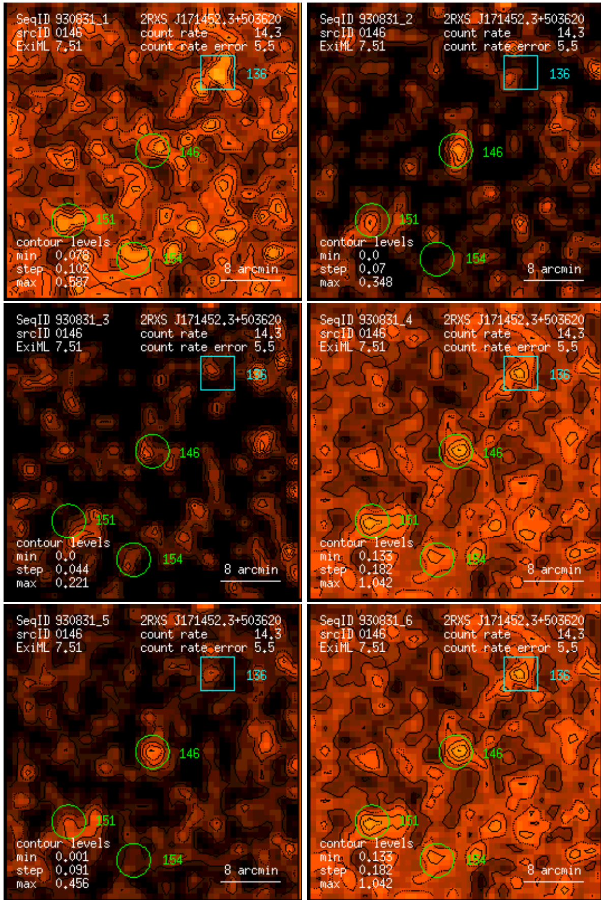
Figure 146: RASS 930831: detection 0146: band rate images, Gaussian filter: (1) PSPC channels 11 – 41, (2) 52 – 90, (3) 91 – 201, (4) 11 – 235, (5) 52 – 201, (6) 11 – 201. Broad band rates in counts/ks. Band rate contour levels in counts/ks/arcmin 2 .
