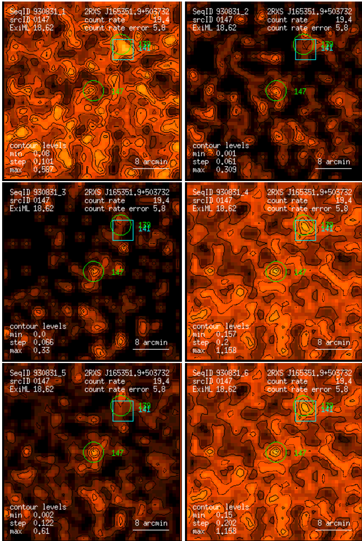
Figure 147: RASS 930831: detection 0147: band rate images, Gaussian filter: (1) PSPC channels 11 – 41, (2) 52 – 90, (3) 91 – 201, (4) 11 – 235, (5) 52 – 201, (6) 11 – 201. Broad band rates in counts/ks. Band rate contour levels in counts/ks/arcmin 2 .
