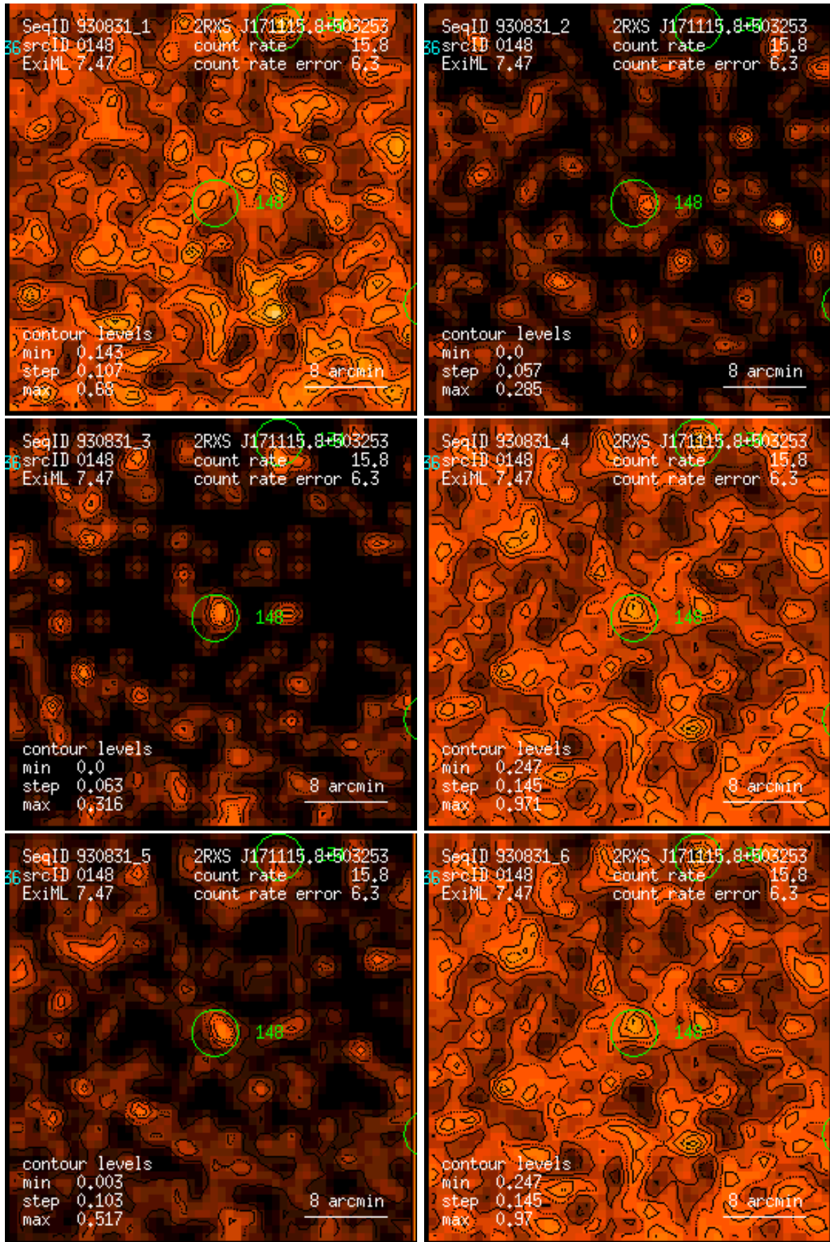
Figure 148: RASS 930831: detection 0148: band rate images, Gaussian filter: (1) PSPC channels 11 – 41, (2) 52 – 90, (3) 91 – 201, (4) 11 – 235, (5) 52 – 201, (6) 11 – 201. Broad band rates in counts/ks. Band rate contour levels in counts/ks/arcmin 2 .
