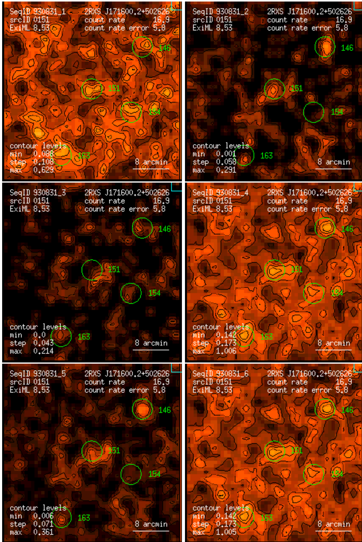
Figure 151: RASS 930831: detection 0151: band rate images, Gaussian filter: (1) PSPC channels 11 – 41, (2) 52 – 90, (3) 91 – 201, (4) 11 – 235, (5) 52 – 201, (6) 11 – 201. Broad band rates in counts/ks. Band rate contour levels in counts/ks/arcmin 2 .
