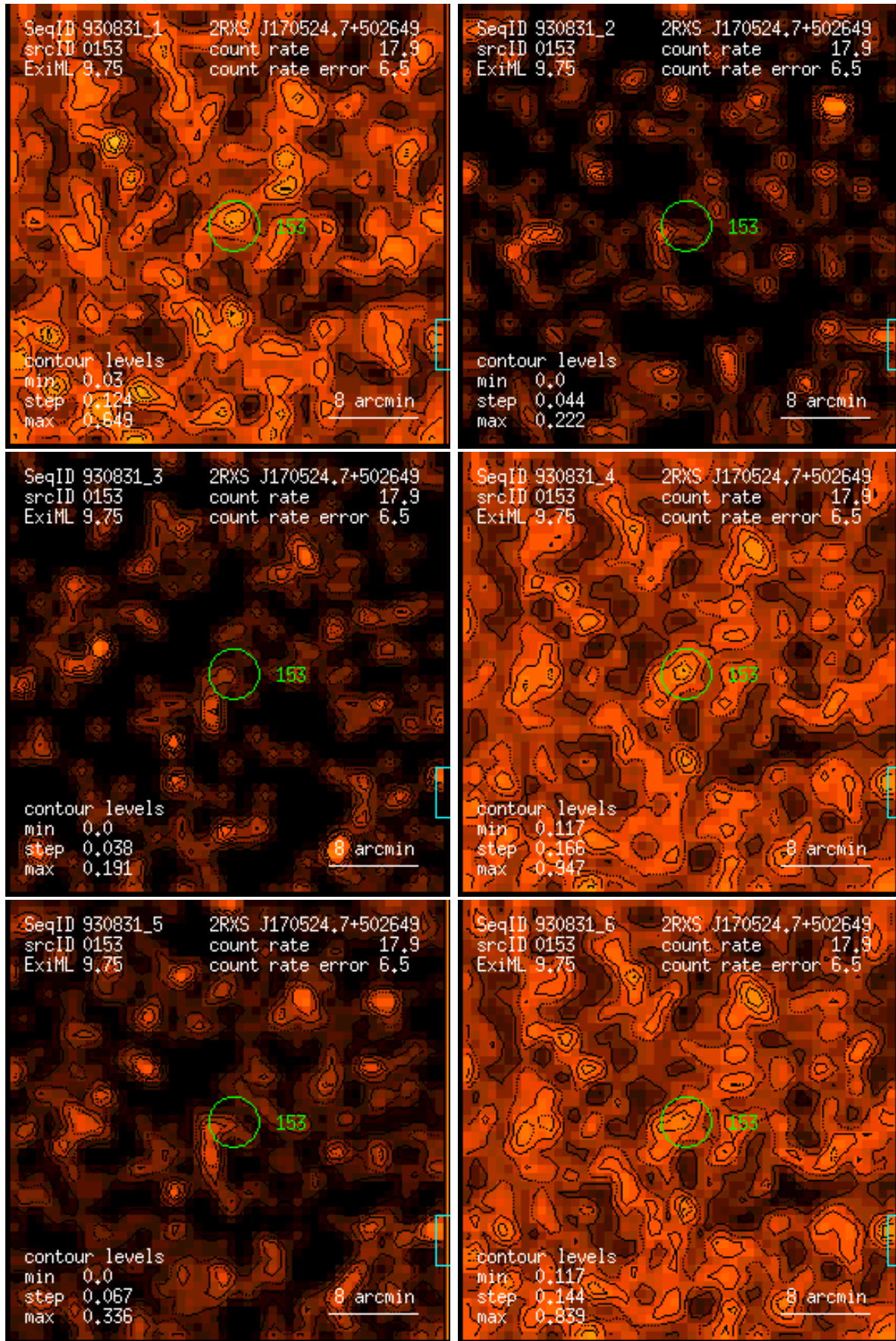
Figure 153: RASS 930831: detection 0153: band rate images, Gaussian filter: (1) PSPC channels 11 – 41, (2) 52 – 90, (3) 91 – 201, (4) 11 – 235, (5) 52 – 201, (6) 11 – 201. Broad band rates in counts/ks. Band rate contour levels in counts/ks/arcmin 2 .
