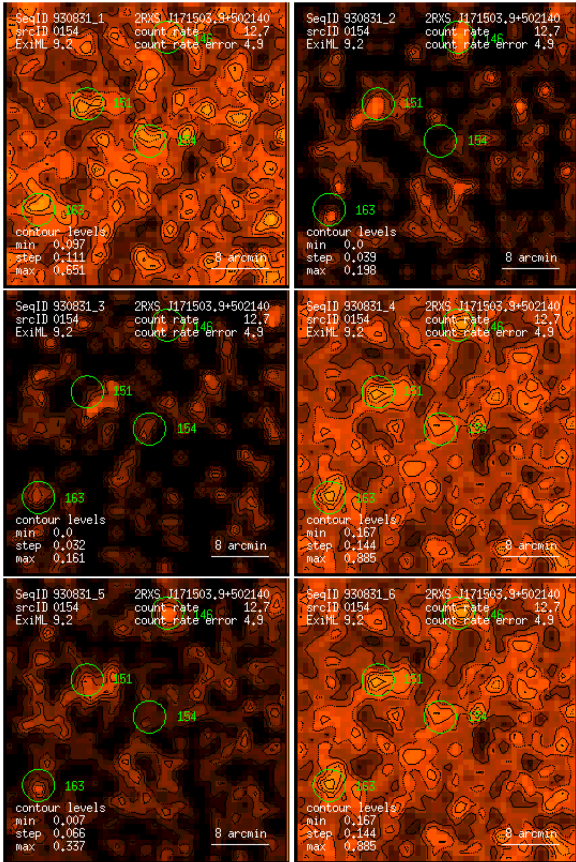
Figure 154: RASS 930831: detection 0154: band rate images, Gaussian filter: (1) PSPC channels 11 – 41, (2) 52 – 90, (3) 91 – 201, (4) 11 – 235, (5) 52 – 201, (6) 11 – 201. Broad band rates in counts/ks. Band rate contour levels in counts/ks/arcmin 2 .
