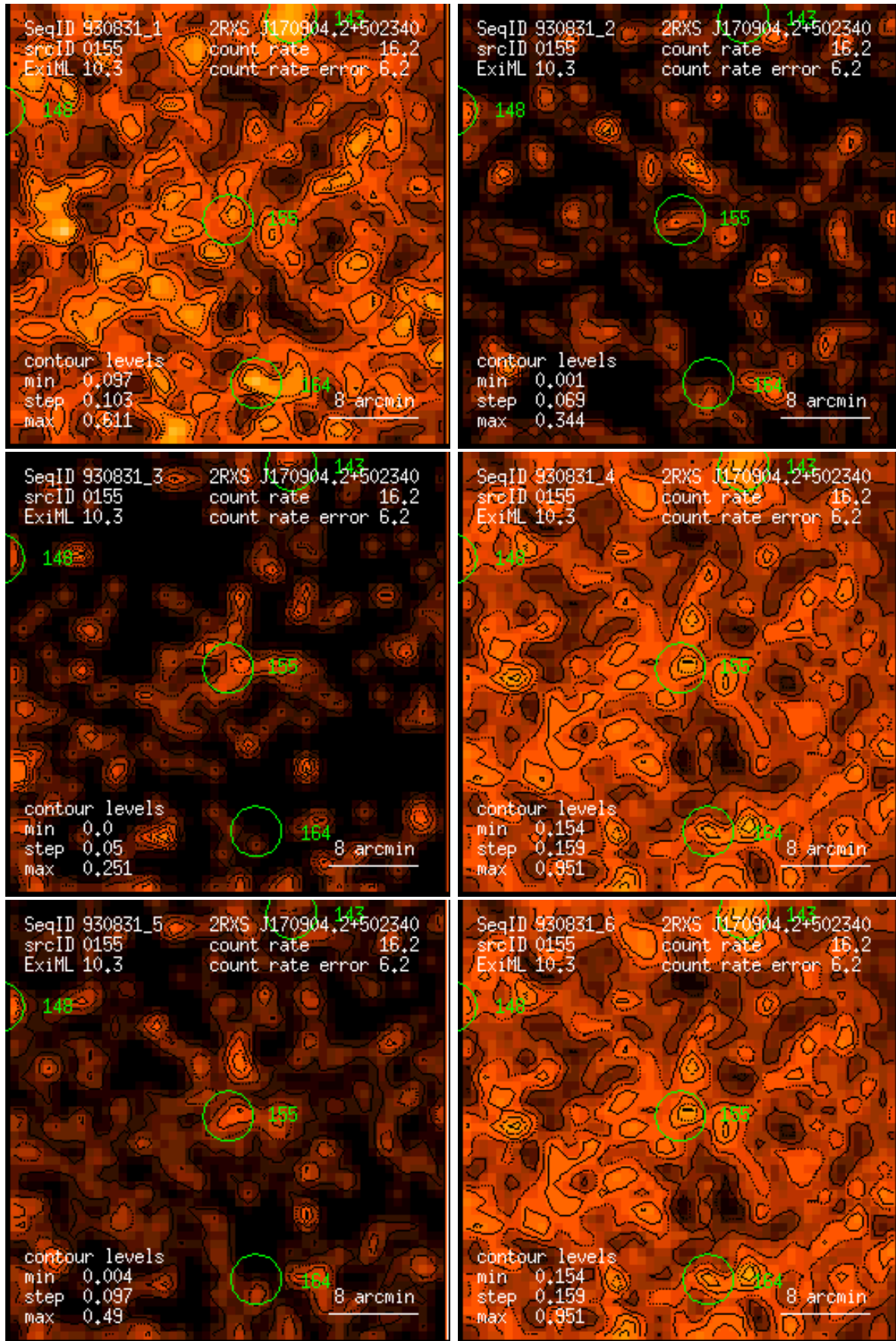
Figure 155: RASS 930831: detection 0155: band rate images, Gaussian filter: (1) PSPC channels 11 – 41, (2) 52 – 90, (3) 91 – 201, (4) 11 – 235, (5) 52 – 201, (6) 11 – 201. Broad band rates in counts/ks. Band rate contour levels in counts/ks/arcmin 2 .
