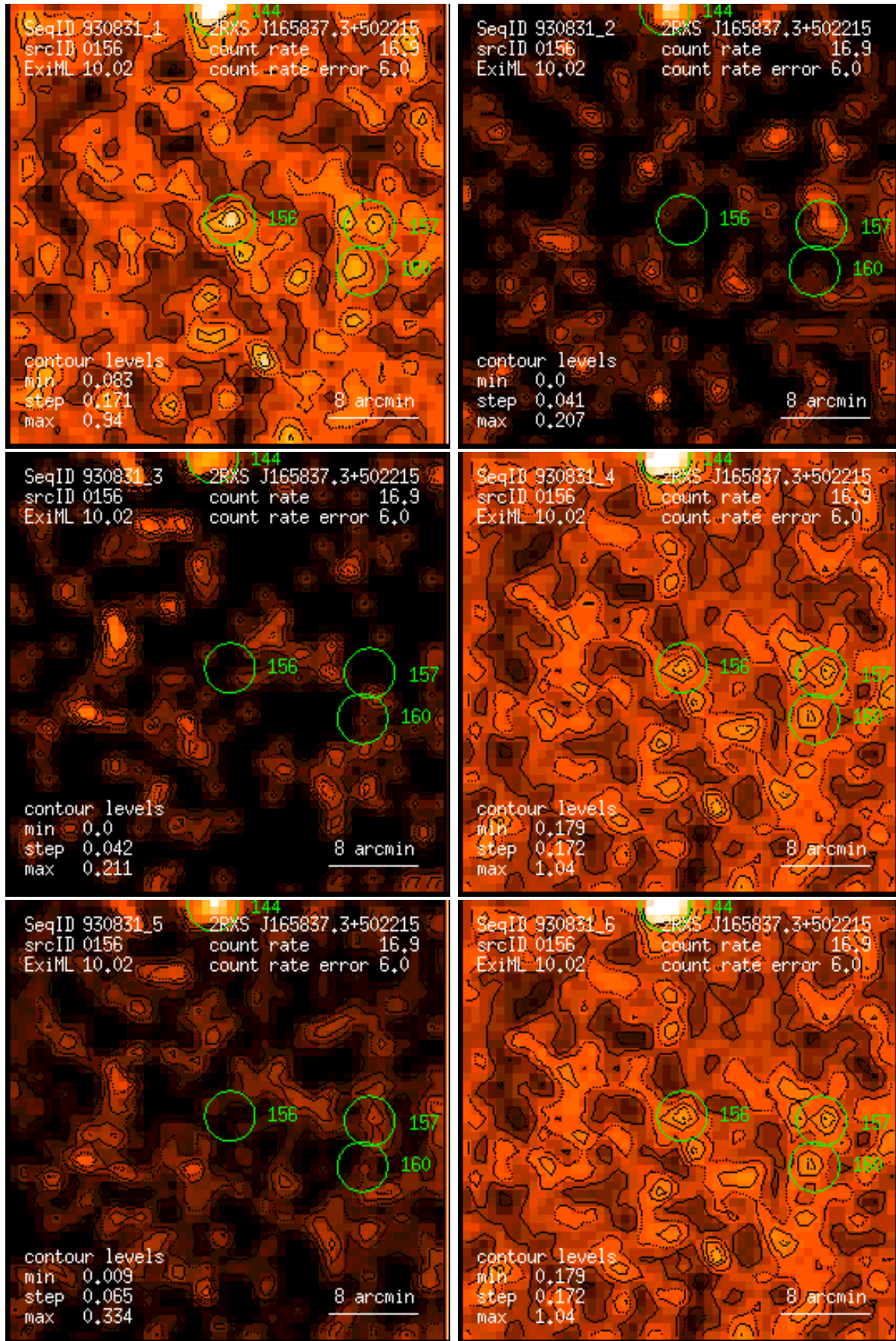
Figure 156: RASS 930831: detection 0156: band rate images, Gaussian filter: (1) PSPC channels 11 – 41, (2) 52 – 90, (3) 91 – 201, (4) 11 – 235, (5) 52 – 201, (6) 11 – 201. Broad band rates in counts/ks. Band rate contour levels in counts/ks/arcmin 2 .
