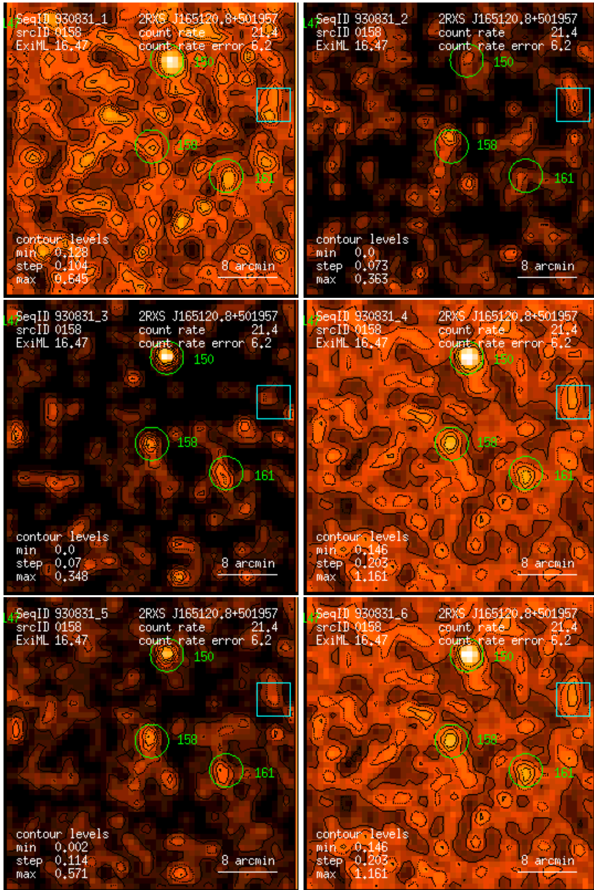
Figure 158: RASS 930831: detection 0158: band rate images, Gaussian filter: (1) PSPC channels 11 – 41, (2) 52 – 90, (3) 91 – 201, (4) 11 – 235, (5) 52 – 201, (6) 11 – 201. Broad band rates in counts/ks. Band rate contour levels in counts/ks/arcmin 2 .
