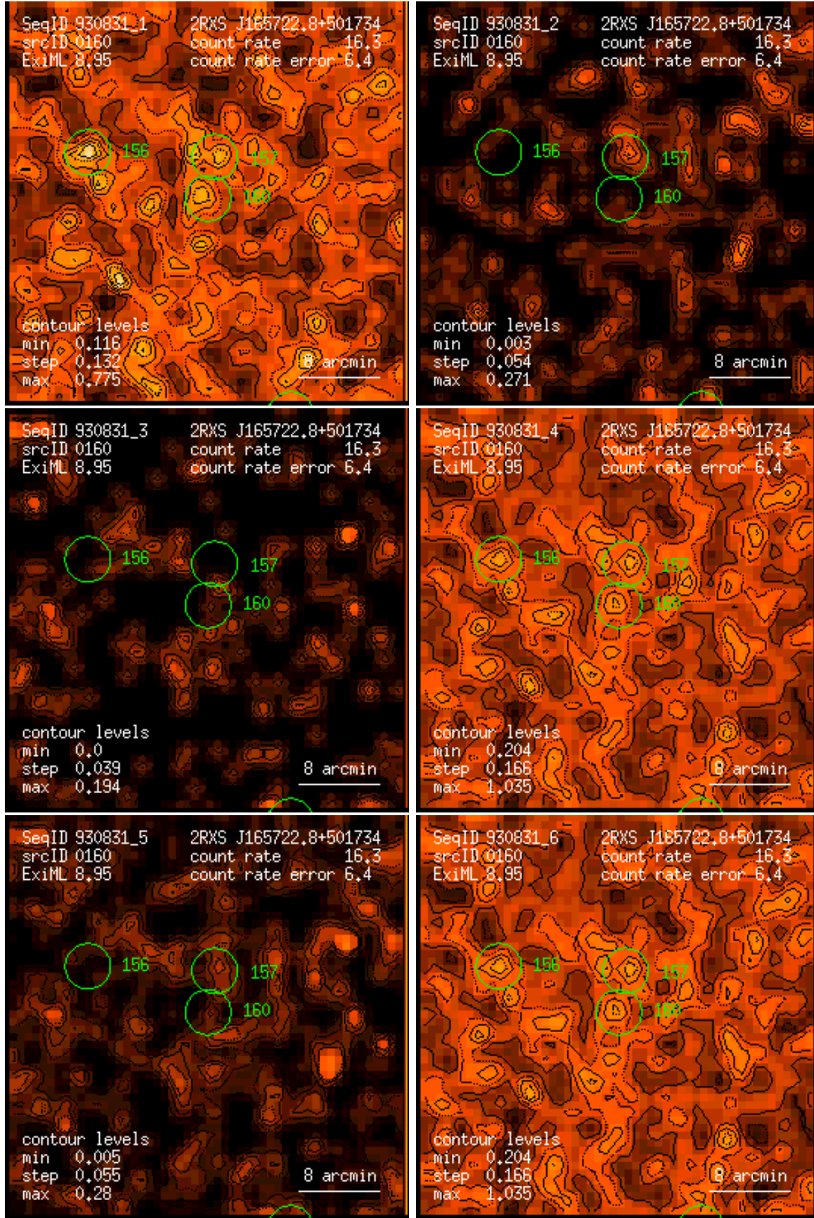
Figure 160: RASS 930831: detection 0160: band rate images, Gaussian filter: (1) PSPC channels 11 – 41, (2) 52 – 90, (3) 91 – 201, (4) 11 – 235, (5) 52 – 201, (6) 11 – 201. Broad band rates in counts/ks. Band rate contour levels in counts/ks/arcmin 2 .
