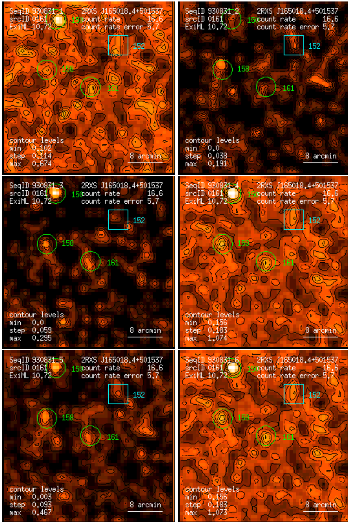
Figure 161: RASS 930831: detection 0161: band rate images, Gaussian filter: (1) PSPC channels 11 – 41, (2) 52 – 90, (3) 91 – 201, (4) 11 – 235, (5) 52 – 201, (6) 11 – 201. Broad band rates in counts/ks. Band rate contour levels in counts/ks/arcmin 2 .
