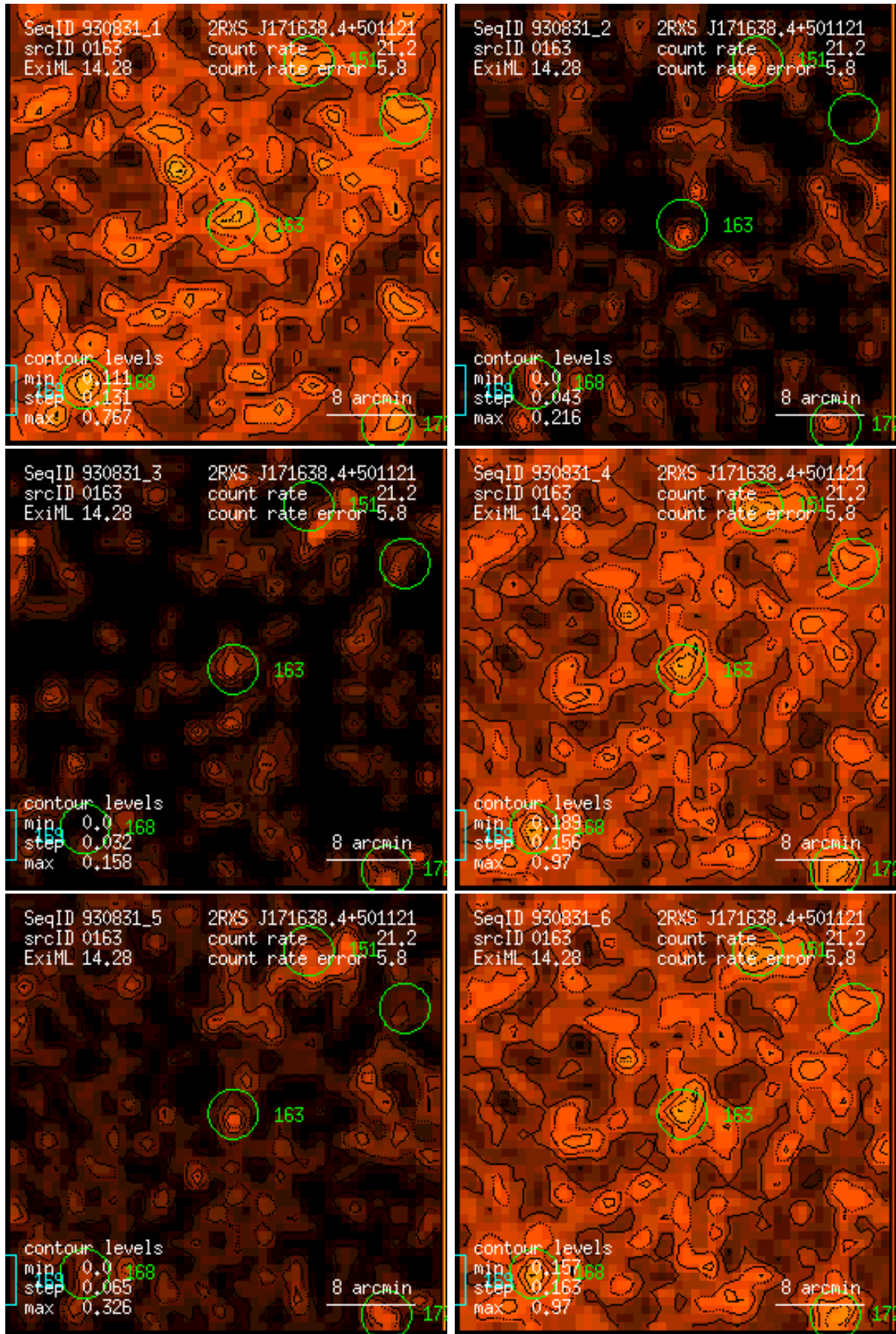
Figure 163: RASS 930831: detection 0163: band rate images, Gaussian filter: (1) PSPC channels 11 – 41, (2) 52 – 90, (3) 91 – 201, (4) 11 – 235, (5) 52 – 201, (6) 11 – 201. Broad band rates in counts/ks. Band rate contour levels in counts/ks/arcmin 2 .
