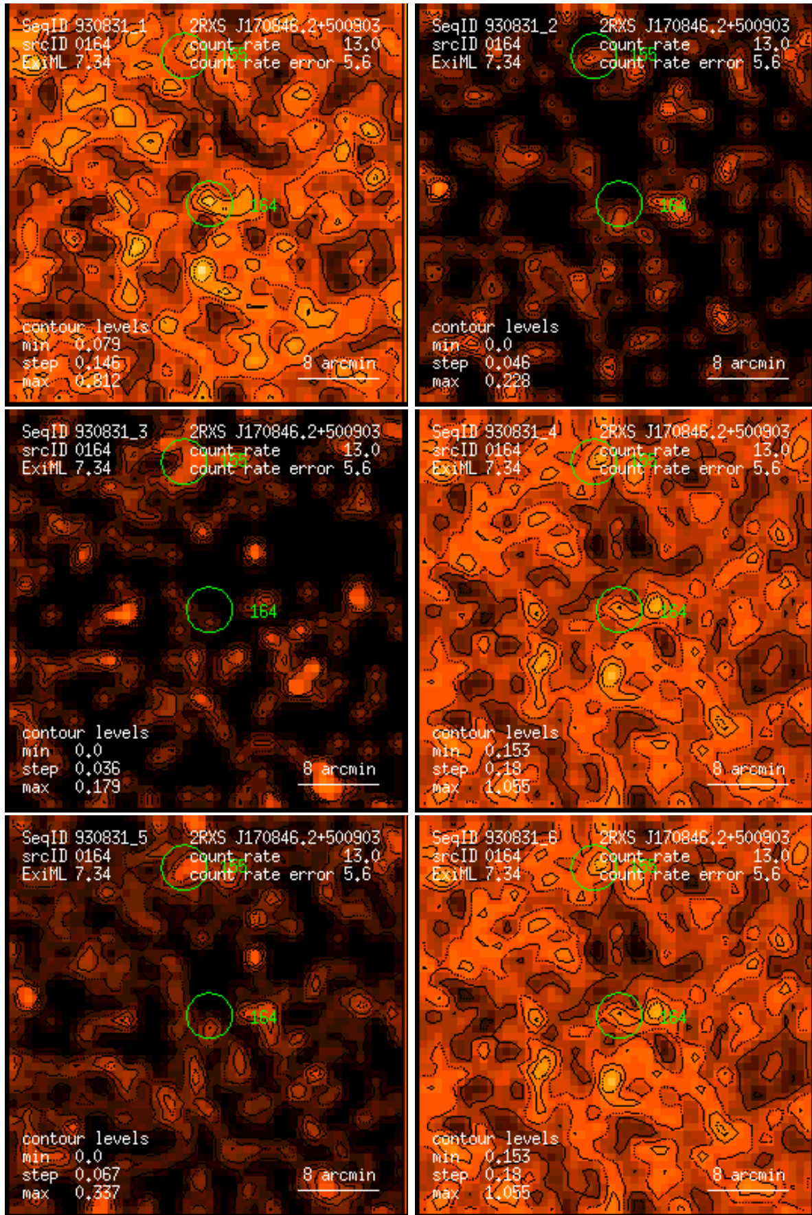
Figure 164: RASS 930831: detection 0164: band rate images, Gaussian filter: (1) PSPC channels 11 – 41, (2) 52 – 90, (3) 91 – 201, (4) 11 – 235, (5) 52 – 201, (6) 11 – 201. Broad band rates in counts/ks. Band rate contour levels in counts/ks/arcmin 2 .
