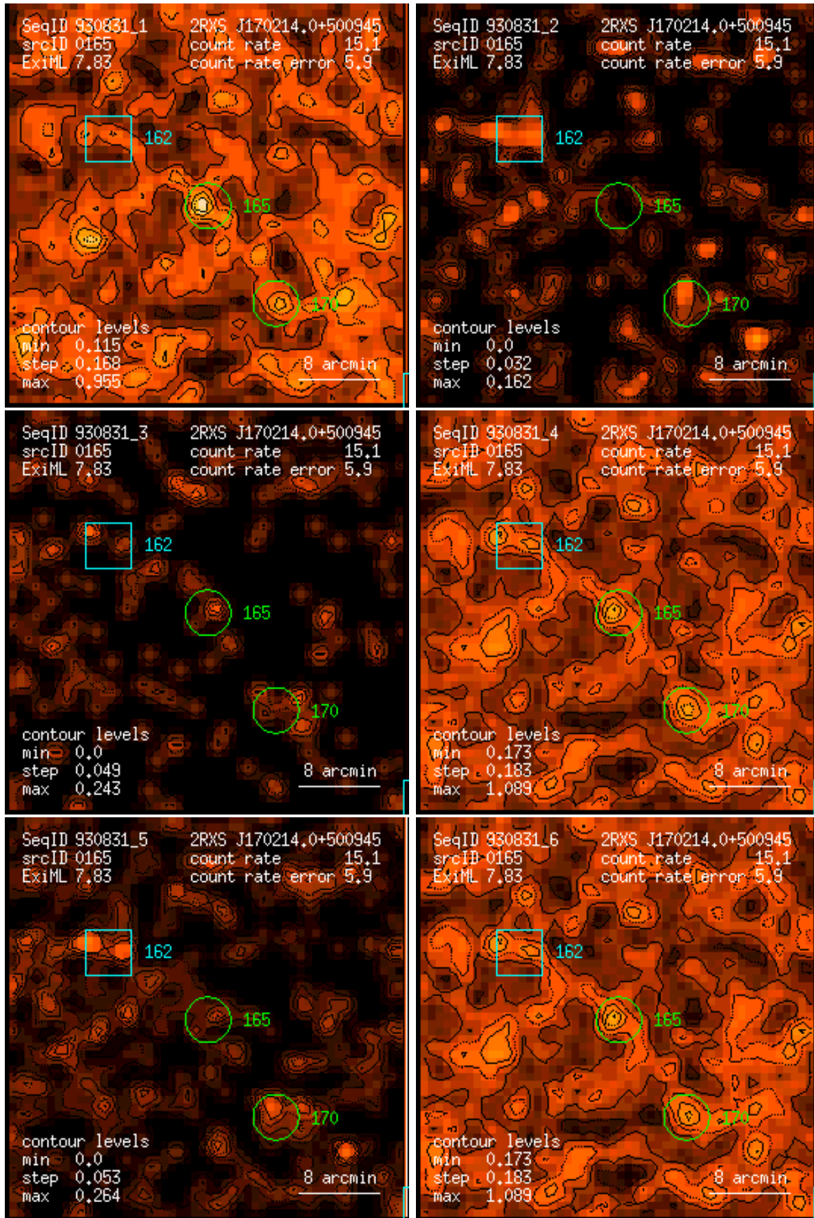
Figure 165: RASS 930831: detection 0165: band rate images, Gaussian filter: (1) PSPC channels 11 – 41, (2) 52 – 90, (3) 91 – 201, (4) 11 – 235, (5) 52 – 201, (6) 11 – 201. Broad band rates in counts/ks. Band rate contour levels in counts/ks/arcmin 2 .
