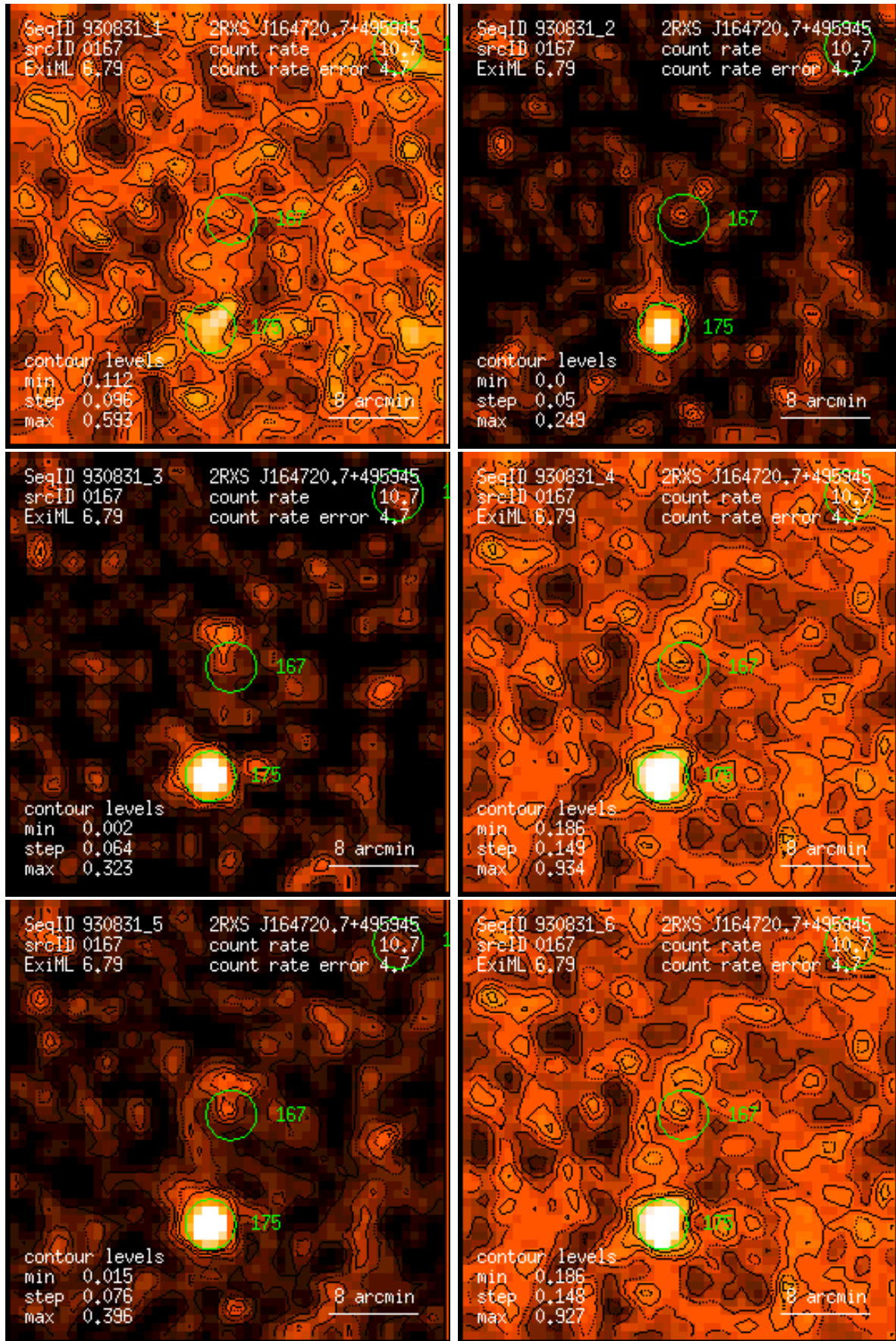
Figure 167: RASS 930831: detection 0167: band rate images, Gaussian filter: (1) PSPC channels 11 – 41, (2) 52 – 90, (3) 91 – 201, (4) 11 – 235, (5) 52 – 201, (6) 11 – 201. Broad band rates in counts/ks. Band rate contour levels in counts/ks/arcmin 2 .
