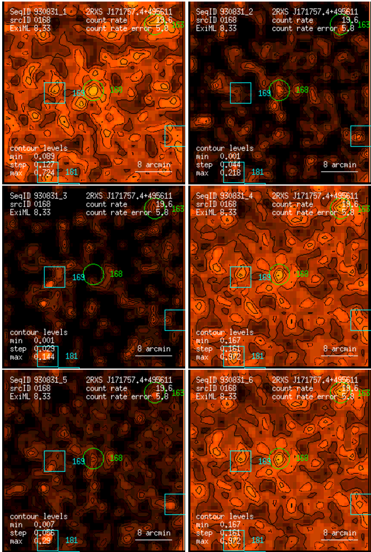
Figure 168: RASS 930831: detection 0168: band rate images, Gaussian filter: (1) PSPC channels 11 – 41, (2) 52 – 90, (3) 91 – 201, (4) 11 – 235, (5) 52 – 201, (6) 11 – 201. Broad band rates in counts/ks. Band rate contour levels in counts/ks/arcmin 2 .
