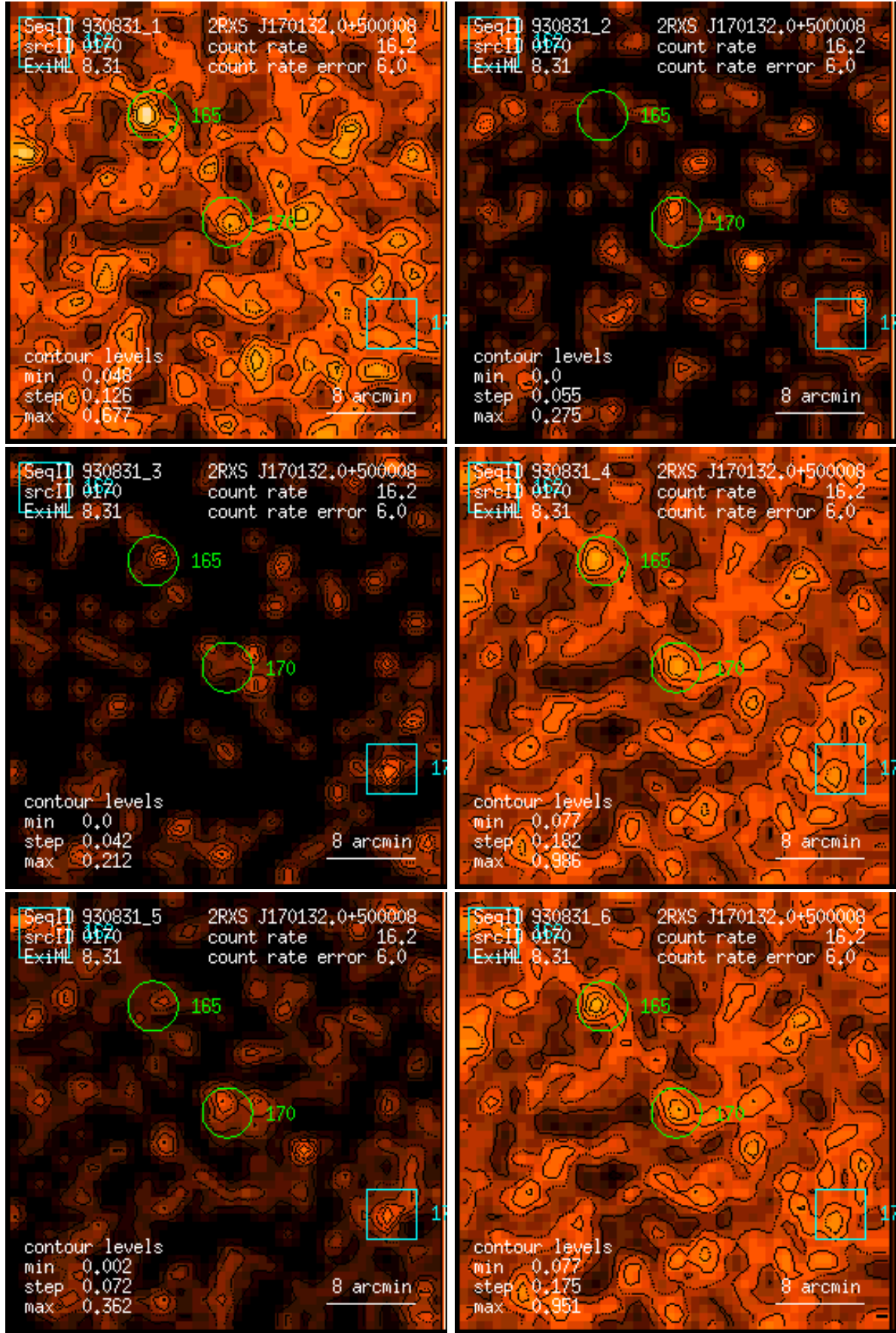
Figure 170: RASS 930831: detection 0170: band rate images, Gaussian filter: (1) PSPC channels 11 – 41, (2) 52 – 90, (3) 91 – 201, (4) 11 – 235, (5) 52 – 201, (6) 11 – 201. Broad band rates in counts/ks. Band rate contour levels in counts/ks/arcmin 2 .
