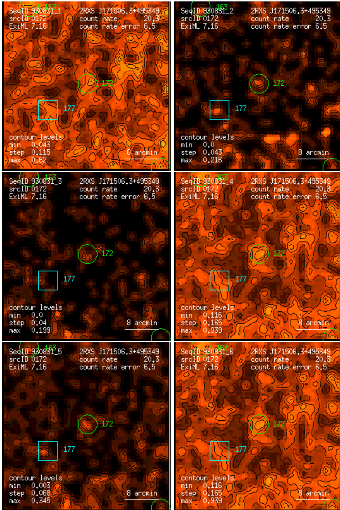
Figure 172: RASS 930831: detection 0172: band rate images, Gaussian filter: (1) PSPC channels 11 – 41, (2) 52 – 90, (3) 91 – 201, (4) 11 – 235, (5) 52 – 201, (6) 11 – 201. Broad band rates in counts/ks. Band rate contour levels in counts/ks/arcmin 2 .
