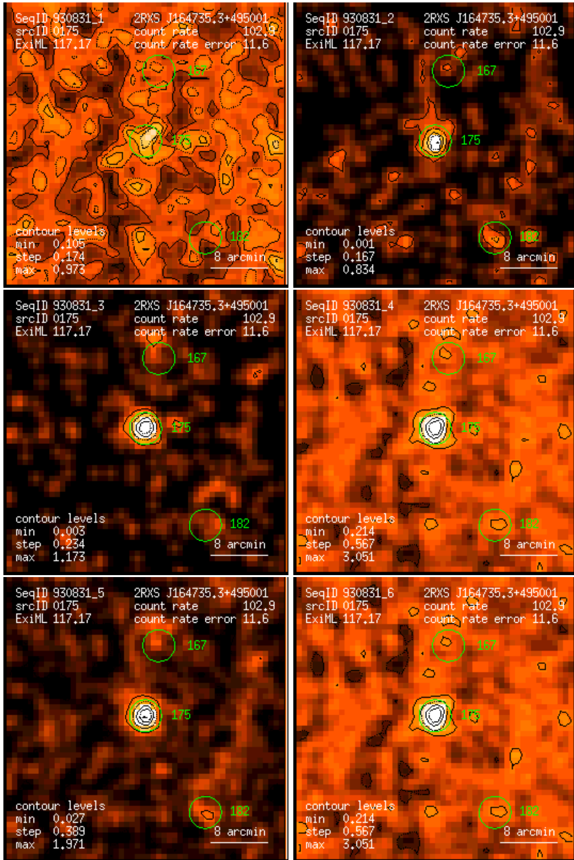
Figure 175: RASS 930831: detection 0175: band rate images, Gaussian filter: (1) PSPC channels 11 – 41, (2) 52 – 90, (3) 91 – 201, (4) 11 – 235, (5) 52 – 201, (6) 11 – 201. Broad band rates in counts/ks. Band rate contour levels in counts/ks/arcmin 2 .
