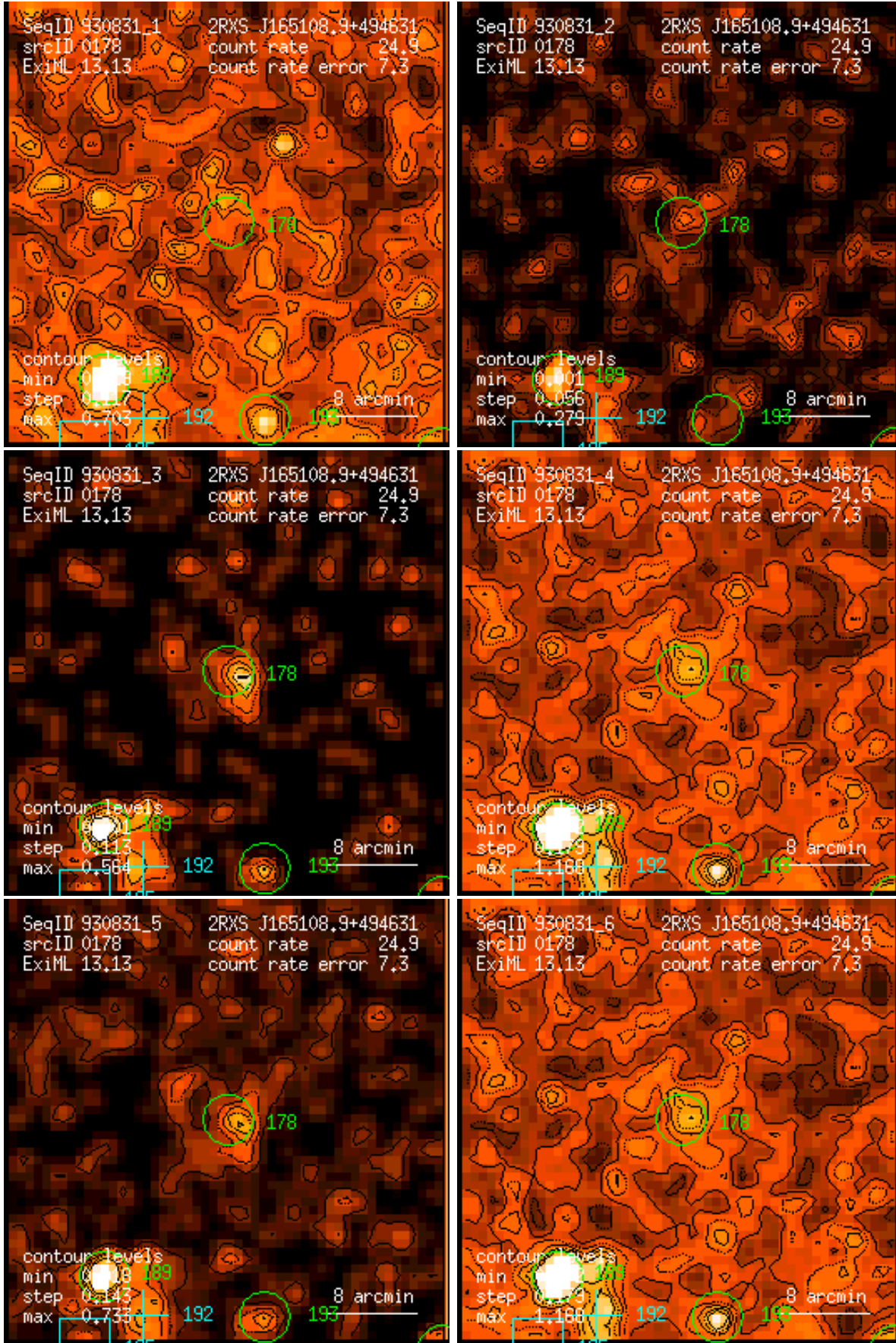
Figure 178: RASS 930831: detection 0178: band rate images, Gaussian filter: (1) PSPC channels 11 – 41, (2) 52 – 90, (3) 91 – 201, (4) 11 – 235, (5) 52 – 201, (6) 11 – 201. Broad band rates in counts/ks. Band rate contour levels in counts/ks/arcmin 2 .
