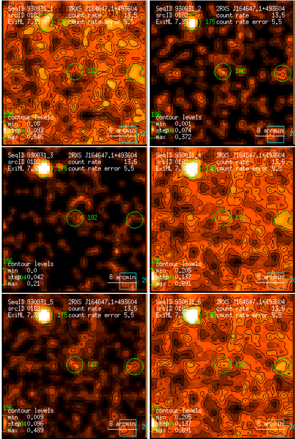
Figure 182: RASS 930831: detection 0182: band rate images, Gaussian filter: (1) PSPC channels 11 – 41, (2) 52 – 90, (3) 91 – 201, (4) 11 – 235, (5) 52 – 201, (6) 11 – 201. Broad band rates in counts/ks. Band rate contour levels in counts/ks/arcmin 2 .
