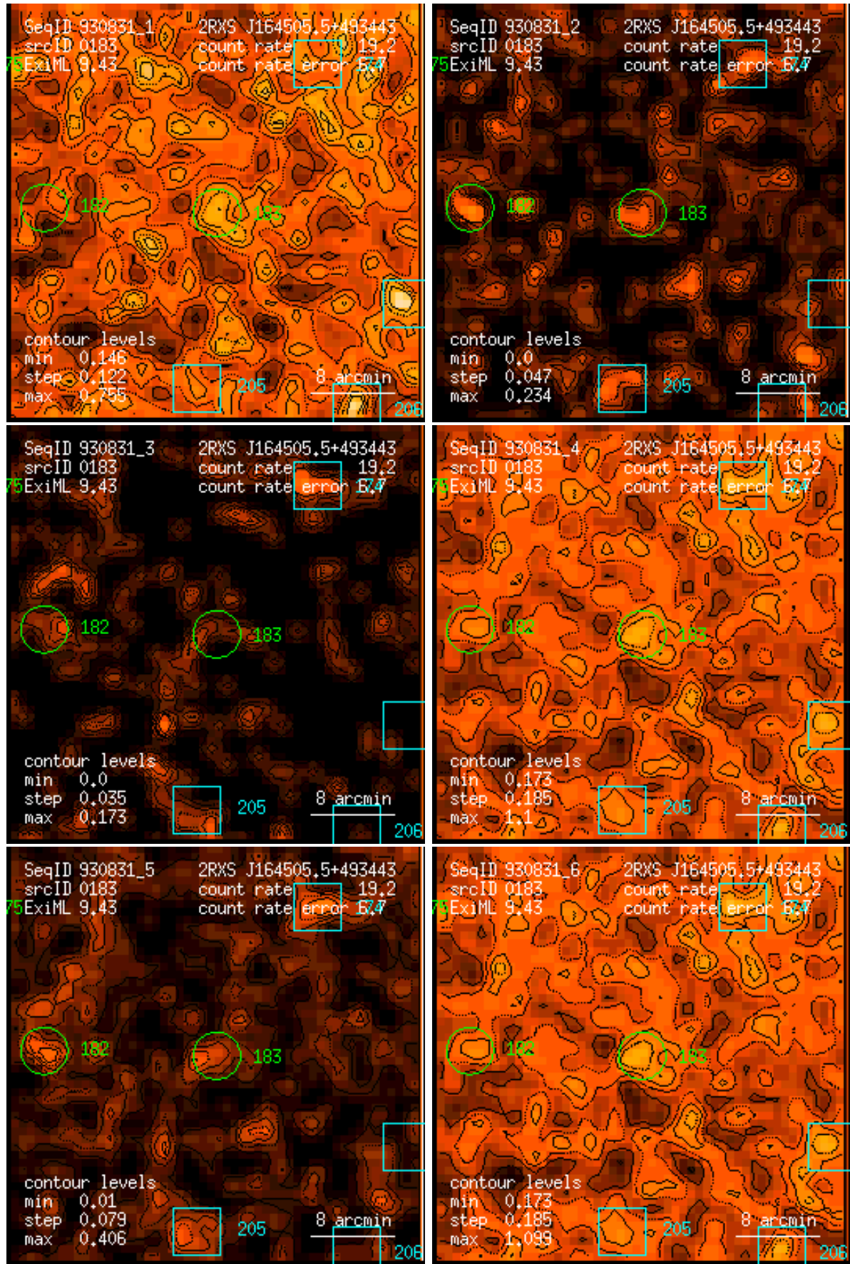
Figure 183: RASS 930831: detection 0183: band rate images, Gaussian filter: (1) PSPC channels 11 – 41, (2) 52 – 90, (3) 91 – 201, (4) 11 – 235, (5) 52 – 201, (6) 11 – 201. Broad band rates in counts/ks. Band rate contour levels in counts/ks/arcmin 2 .
