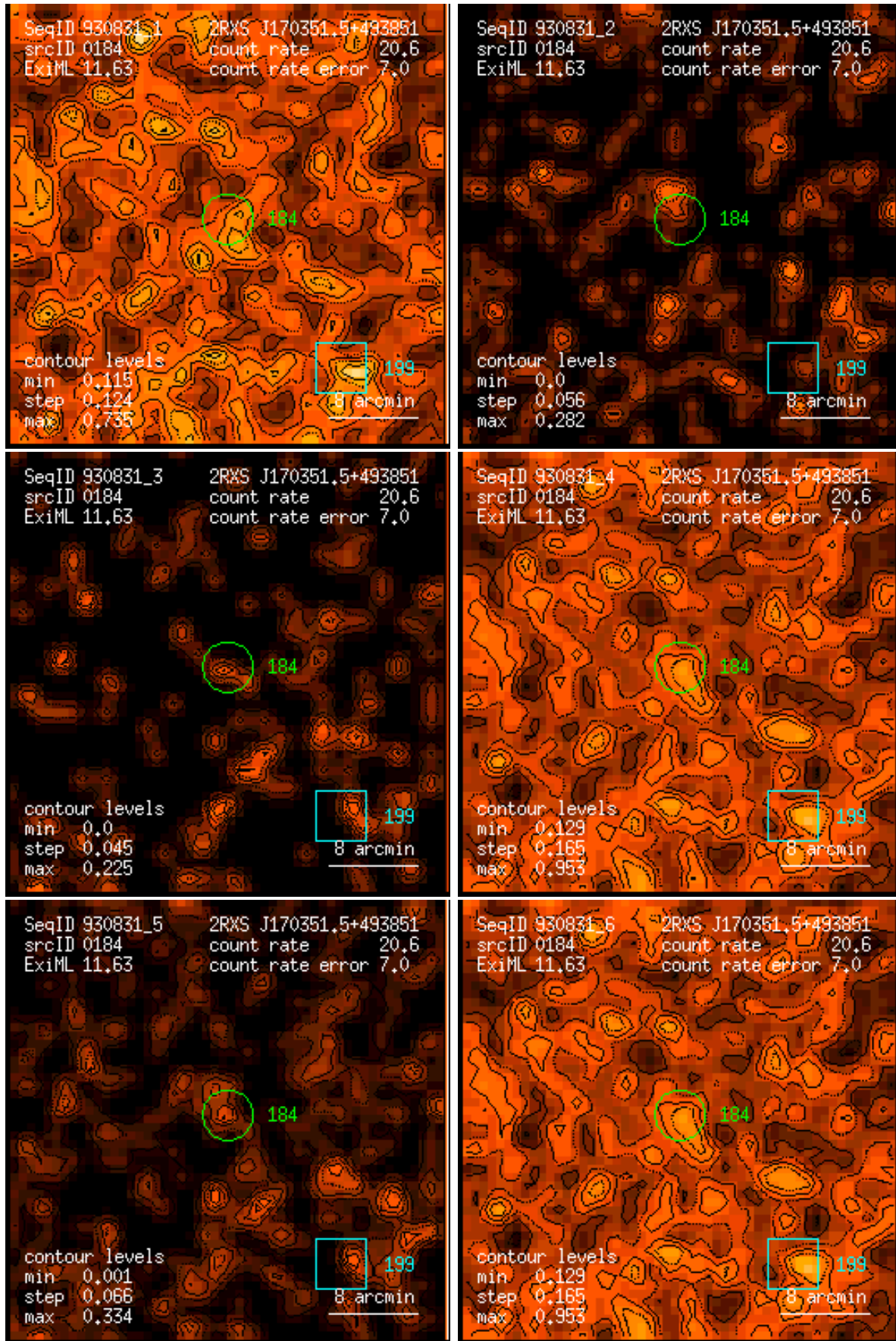
Figure 184: RASS 930831: detection 0184: band rate images, Gaussian filter: (1) PSPC channels 11 – 41, (2) 52 – 90, (3) 91 – 201, (4) 11 – 235, (5) 52 – 201, (6) 11 – 201. Broad band rates in counts/ks. Band rate contour levels in counts/ks/arcmin 2 .
