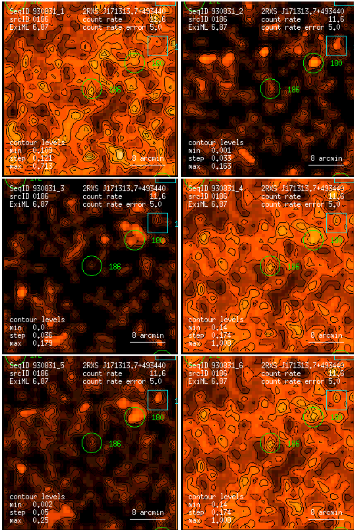
Figure 186: RASS 930831: detection 0186: band rate images, Gaussian filter: (1) PSPC channels 11 – 41, (2) 52 – 90, (3) 91 – 201, (4) 11 – 235, (5) 52 – 201, (6) 11 – 201. Broad band rates in counts/ks. Band rate contour levels in counts/ks/arcmin 2 .
