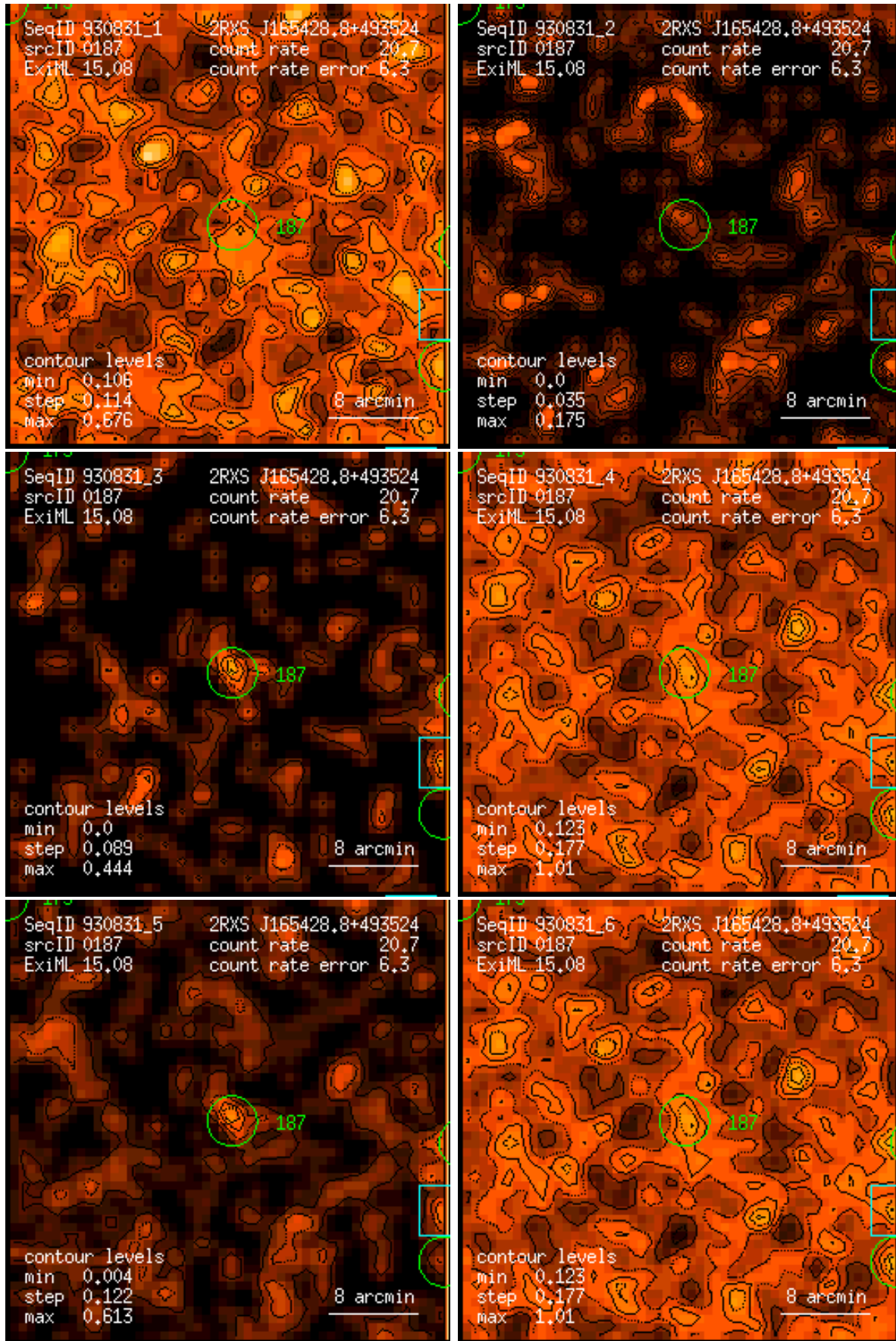
Figure 187: RASS 930831: detection 0187: band rate images, Gaussian filter: (1) PSPC channels 11 – 41, (2) 52 – 90, (3) 91 – 201, (4) 11 – 235, (5) 52 – 201, (6) 11 – 201. Broad band rates in counts/ks. Band rate contour levels in counts/ks/arcmin 2 .
