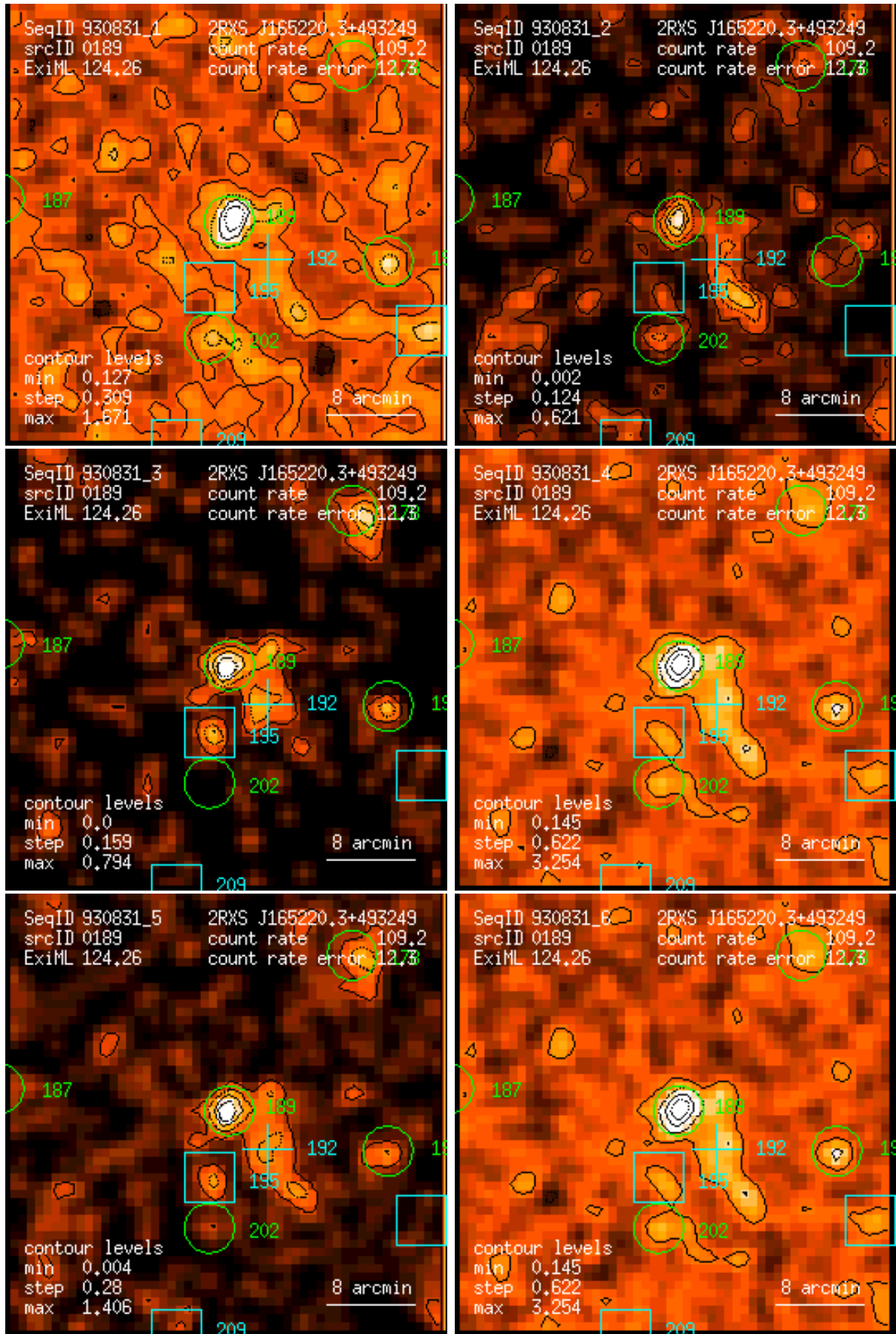
Figure 189: RASS 930831: detection 0189: band rate images, Gaussian filter: (1) PSPC channels 11 – 41, (2) 52 – 90, (3) 91 – 201, (4) 11 – 235, (5) 52 – 201, (6) 11 – 201. Broad band rates in counts/ks. Band rate contour levels in counts/ks/arcmin 2 .
