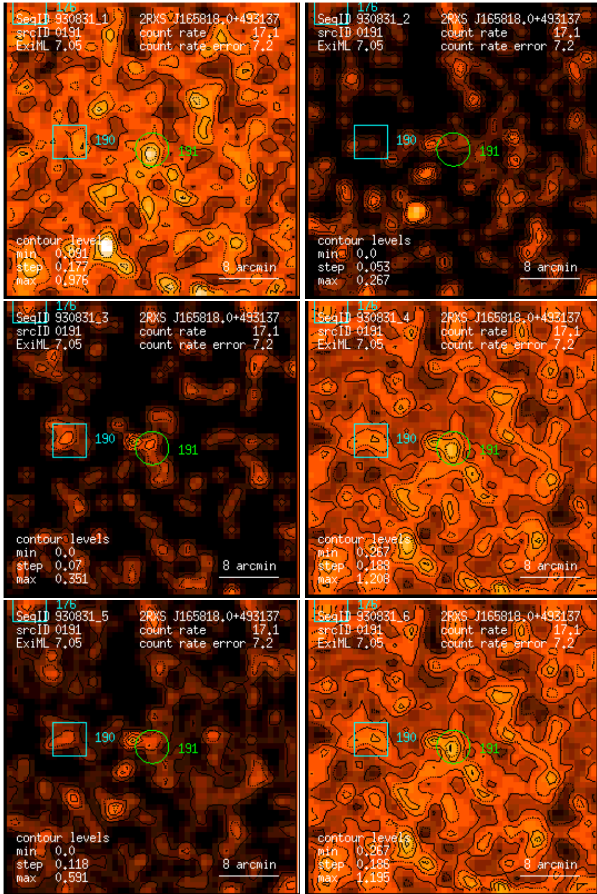
Figure 191: RASS 930831: detection 0191: band rate images, Gaussian filter: (1) PSPC channels 11 – 41, (2) 52 – 90, (3) 91 – 201, (4) 11 – 235, (5) 52 – 201, (6) 11 – 201. Broad band rates in counts/ks. Band rate contour levels in counts/ks/arcmin 2 .
