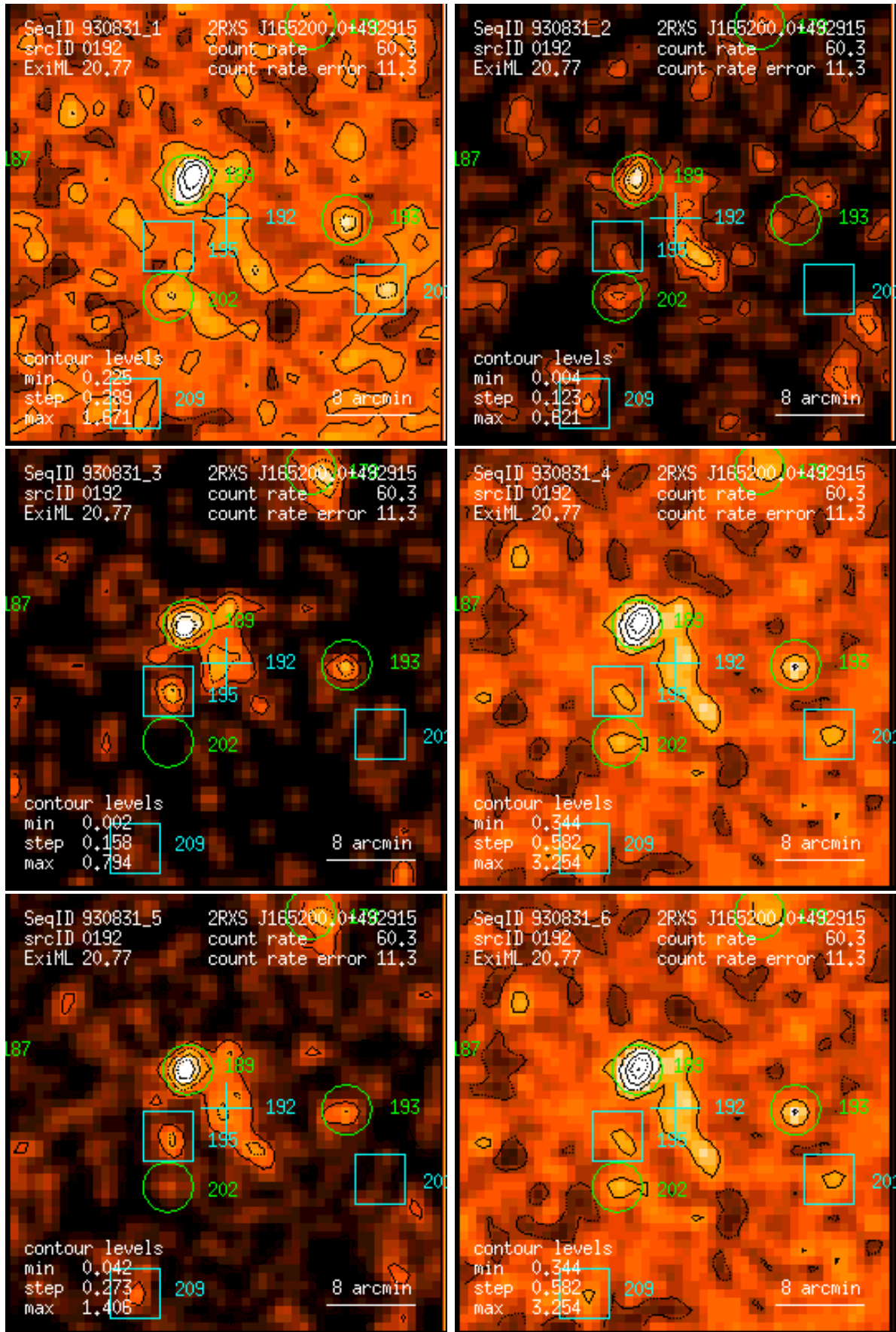
Figure 192: RASS 930831: detection 0192: band rate images, Gaussian filter: (1) PSPC channels 11 – 41, (2) 52 – 90, (3) 91 – 201, (4) 11 – 235, (5) 52 – 201, (6) 11 – 201. Broad band rates in counts/ks. Band rate contour levels in counts/ks/arcmin 2 .
