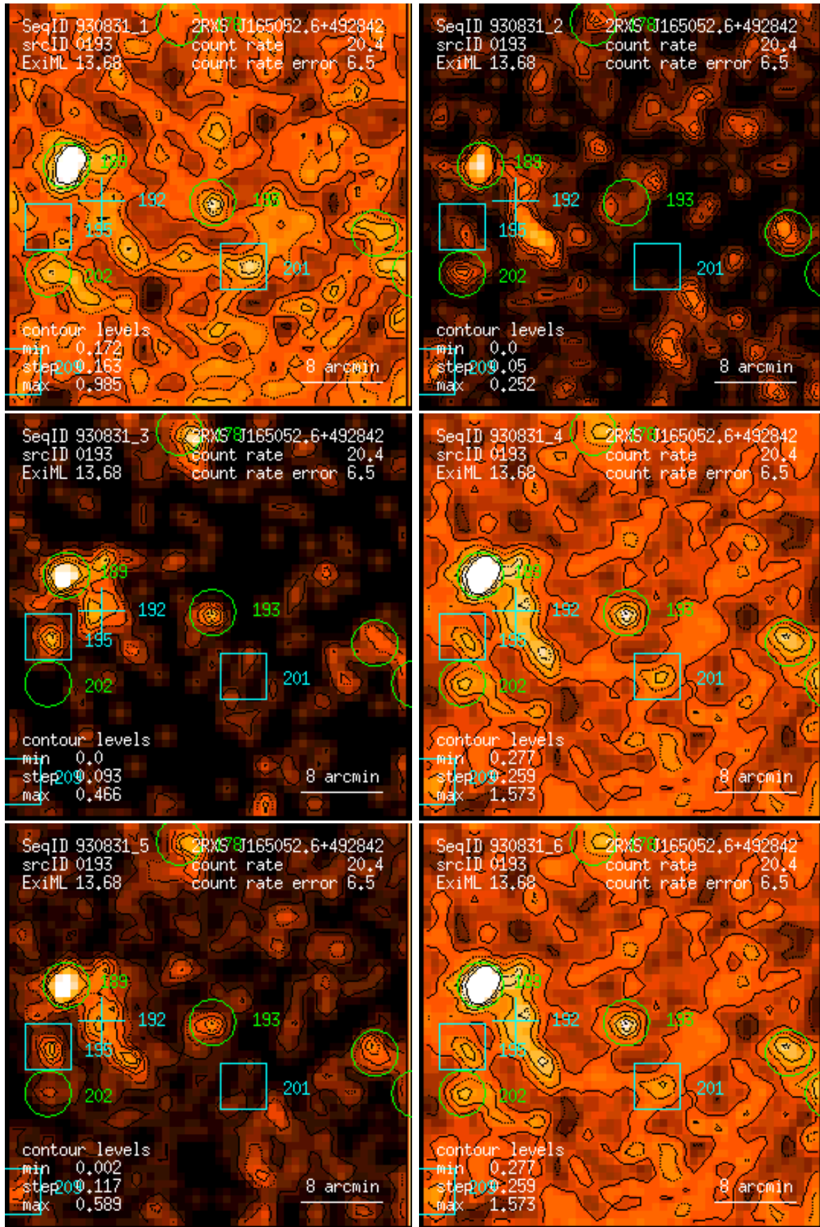
Figure 193: RASS 930831: detection 0193: band rate images, Gaussian filter: (1) PSPC channels 11 – 41, (2) 52 – 90, (3) 91 – 201, (4) 11 – 235, (5) 52 – 201, (6) 11 – 201. Broad band rates in counts/ks. Band rate contour levels in counts/ks/arcmin 2 .
