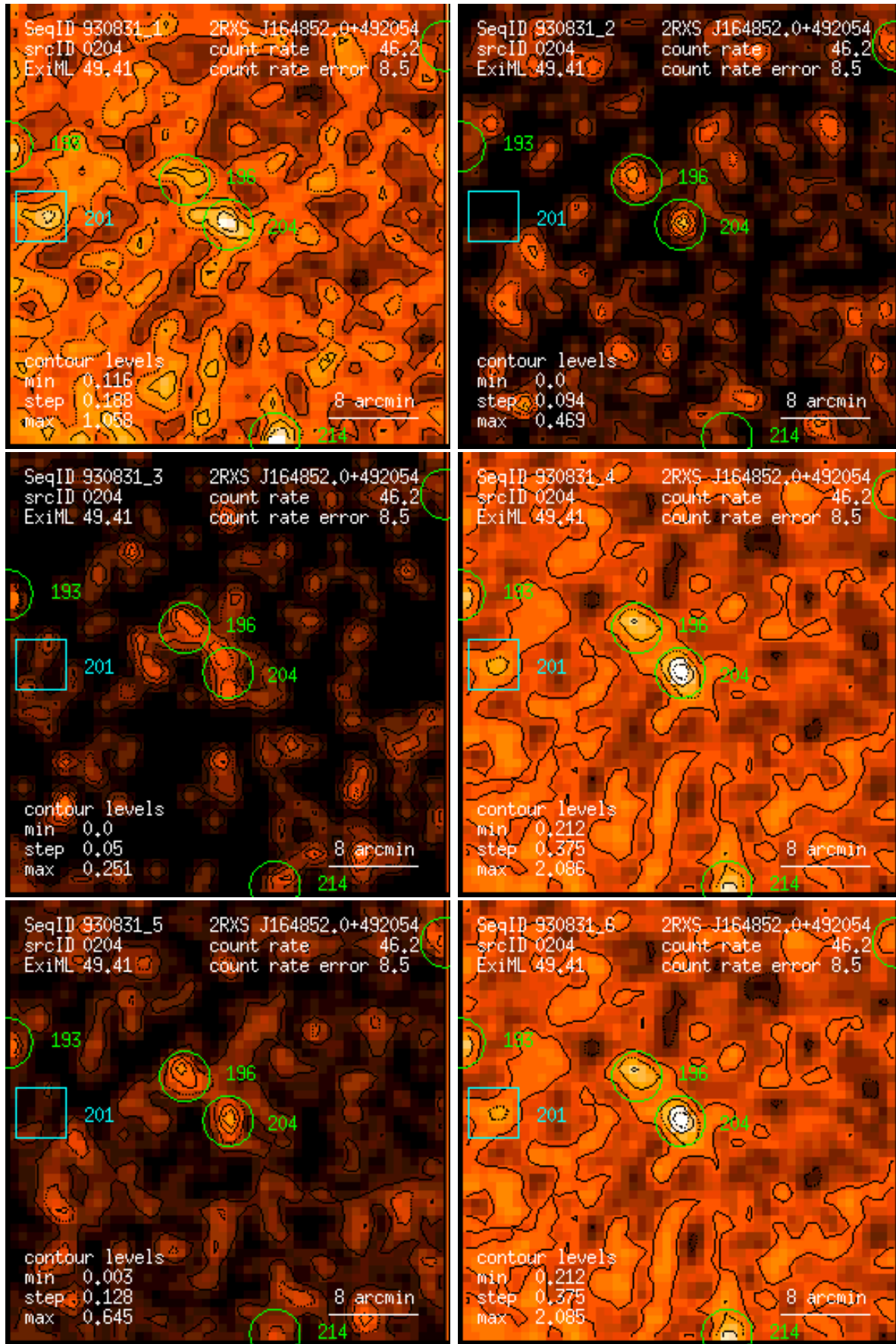
Figure 204: RASS 930831: detection 0204: band rate images, Gaussian filter: (1) PSPC channels 11 – 41, (2) 52 – 90, (3) 91 – 201, (4) 11 – 235, (5) 52 – 201, (6) 11 – 201. Broad band rates in counts/ks. Band rate contour levels in counts/ks/arcmin 2 .
