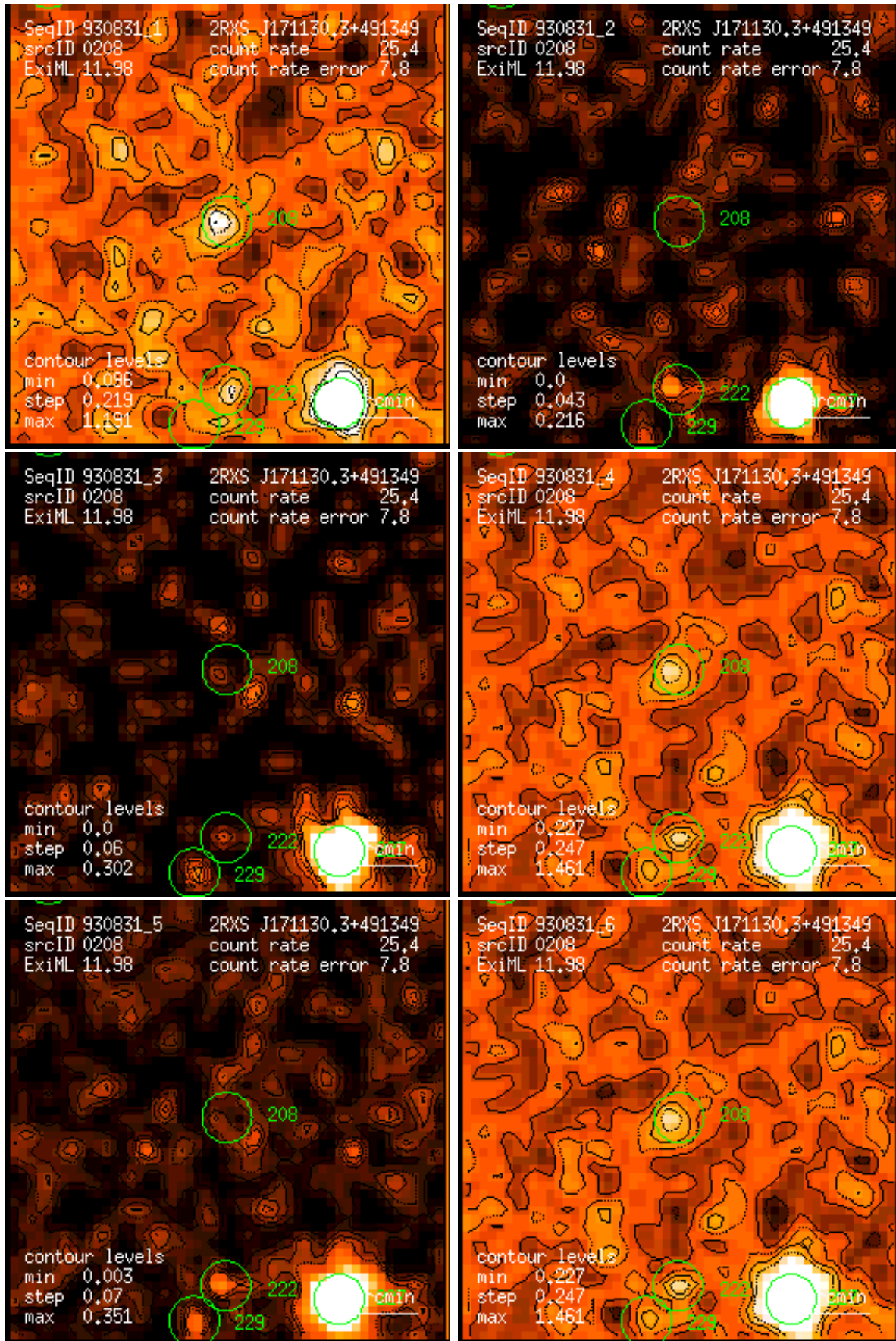
Figure 208: RASS 930831: detection 0208: band rate images, Gaussian filter: (1) PSPC channels 11 – 41, (2) 52 – 90, (3) 91 – 201, (4) 11 – 235, (5) 52 – 201, (6) 11 – 201. Broad band rates in counts/ks. Band rate contour levels in counts/ks/arcmin 2 .
