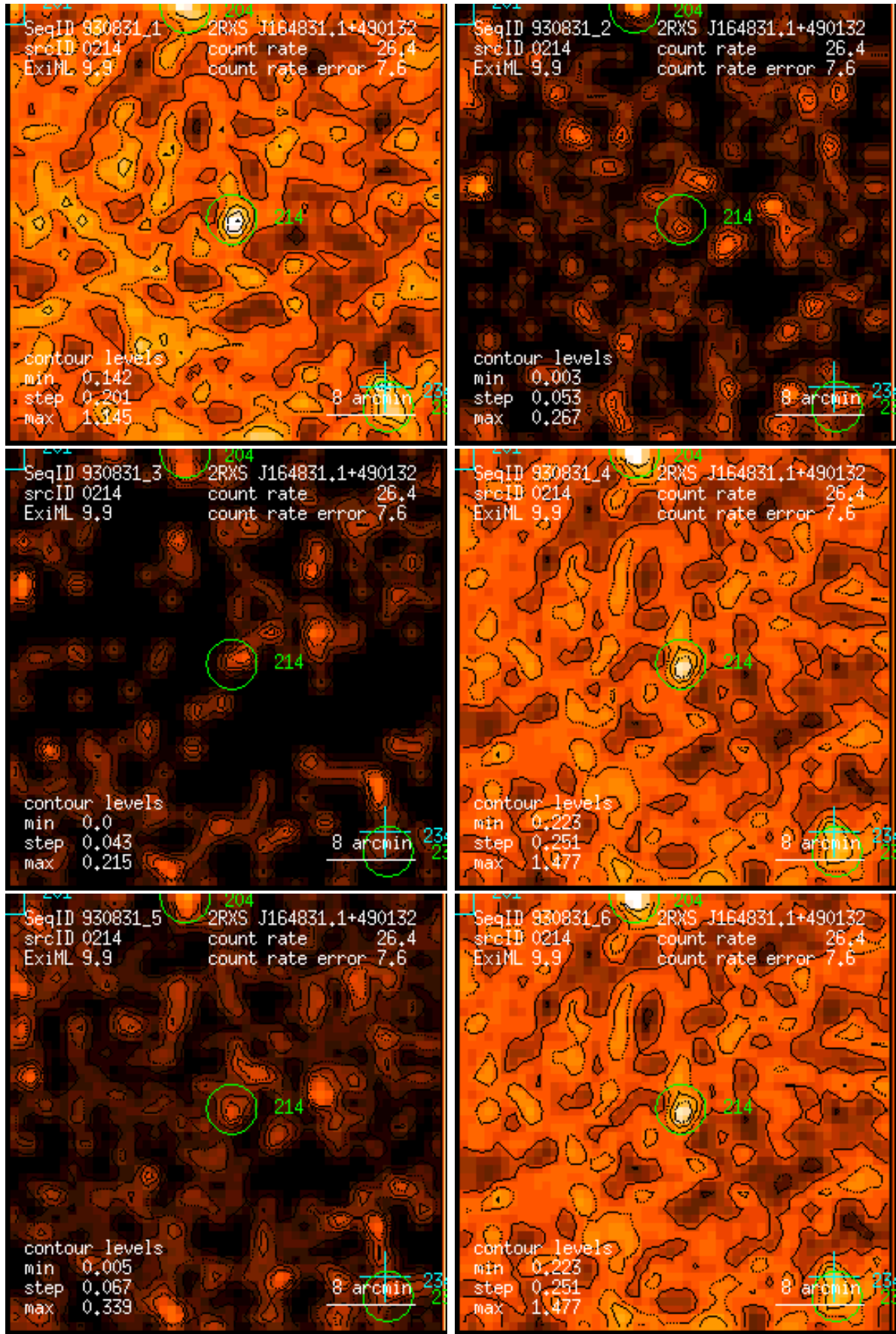
Figure 214: RASS 930831: detection 0214: band rate images, Gaussian filter: (1) PSPC channels 11 – 41, (2) 52 – 90, (3) 91 – 201, (4) 11 – 235, (5) 52 – 201, (6) 11 – 201. Broad band rates in counts/ks. Band rate contour levels in counts/ks/arcmin 2 .
