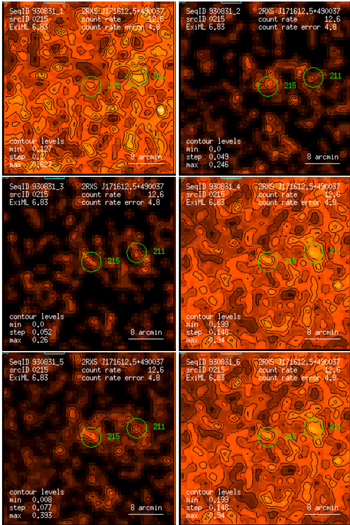
Figure 215: RASS 930831: detection 0215: band rate images, Gaussian filter: (1) PSPC channels 11 – 41, (2) 52 – 90, (3) 91 – 201, (4) 11 – 235, (5) 52 – 201, (6) 11 – 201. Broad band rates in counts/ks. Band rate contour levels in counts/ks/arcmin 2 .
