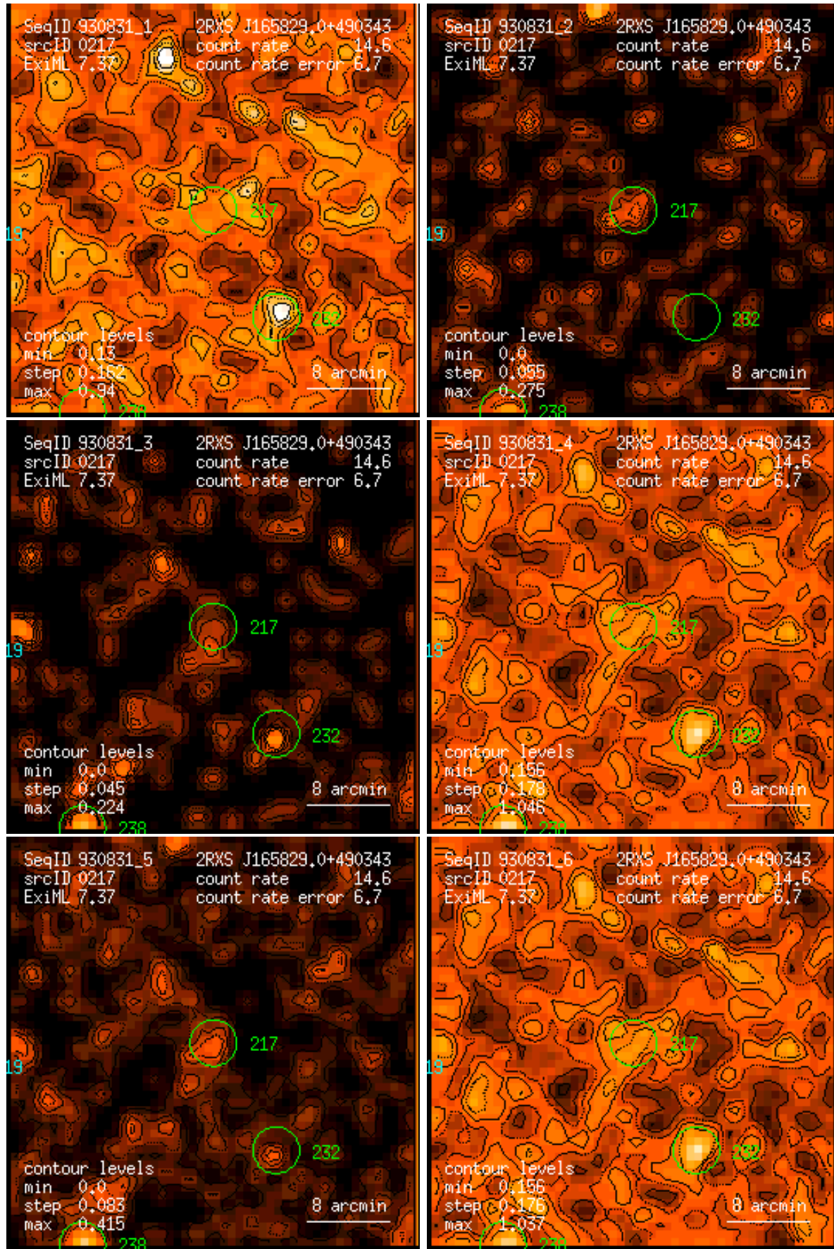
Figure 217: RASS 930831: detection 0217: band rate images, Gaussian filter: (1) PSPC channels 11 – 41, (2) 52 – 90, (3) 91 – 201, (4) 11 – 235, (5) 52 – 201, (6) 11 – 201. Broad band rates in counts/ks. Band rate contour levels in counts/ks/arcmin 2 .
