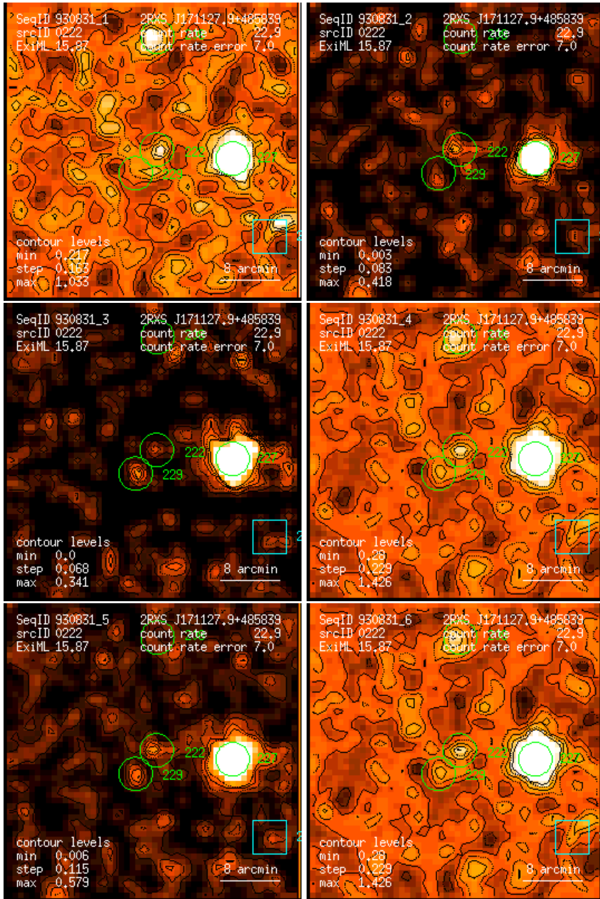
Figure 222: RASS 930831: detection 0222: band rate images, Gaussian filter: (1) PSPC channels 11 – 41, (2) 52 – 90, (3) 91 – 201, (4) 11 – 235, (5) 52 – 201, (6) 11 – 201. Broad band rates in counts/ks. Band rate contour levels in counts/ks/arcmin 2 .
