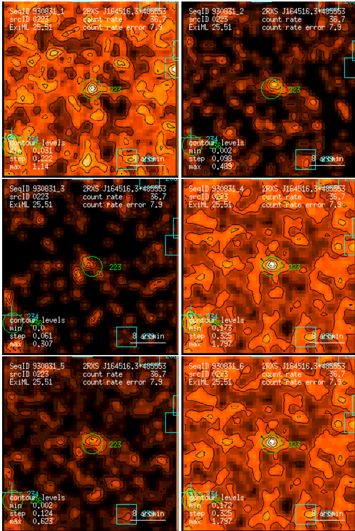
Figure 223: RASS 930831: detection 0223: band rate images, Gaussian filter: (1) PSPC channels 11 – 41, (2) 52 – 90, (3) 91 – 201, (4) 11 – 235, (5) 52 – 201, (6) 11 – 201. Broad band rates in counts/ks. Band rate contour levels in counts/ks/arcmin 2 .
