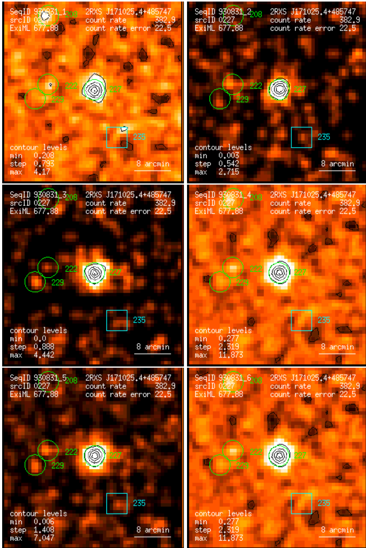
Figure 227: RASS 930831: detection 0227: band rate images, Gaussian filter: (1) PSPC channels 11 – 41, (2) 52 – 90, (3) 91 – 201, (4) 11 – 235, (5) 52 – 201, (6) 11 – 201. Broad band rates in counts/ks. Band rate contour levels in counts/ks/arcmin 2 .
