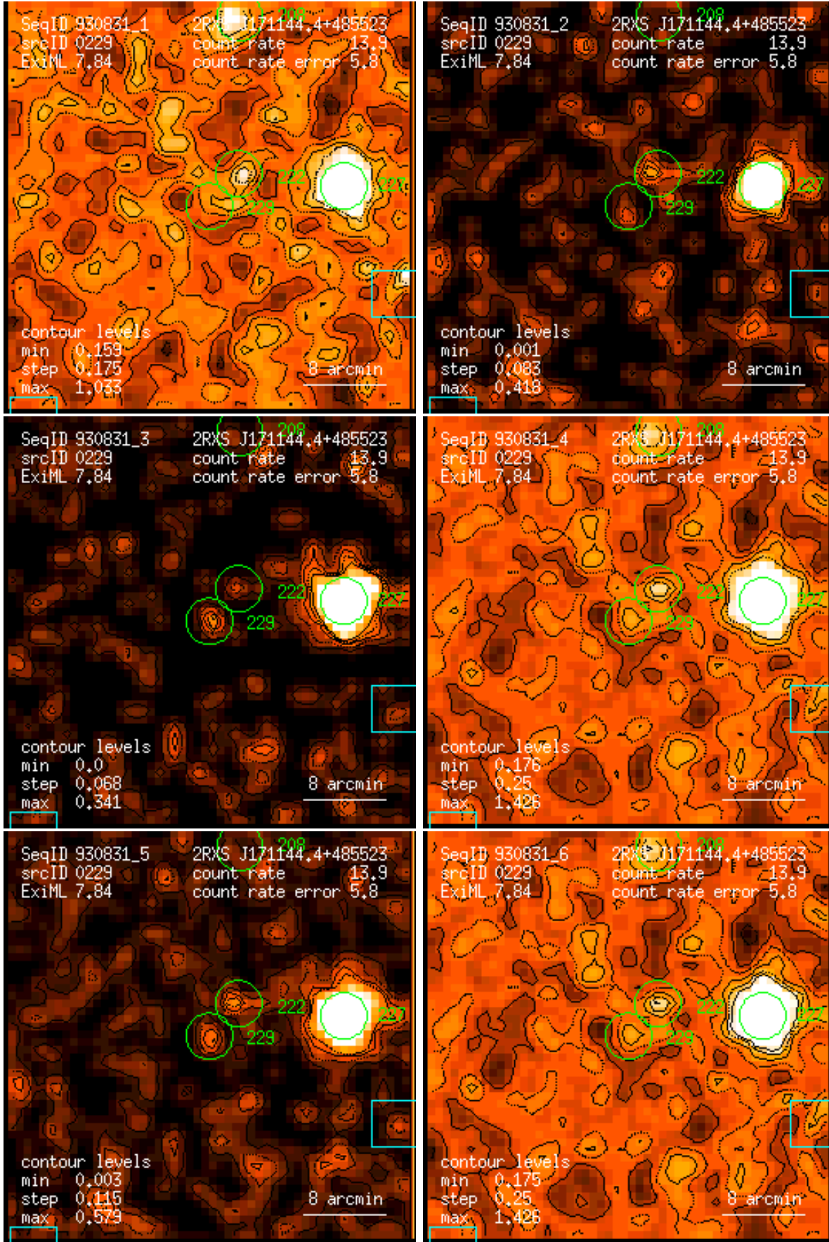
Figure 229: RASS 930831: detection 0229: band rate images, Gaussian filter: (1) PSPC channels 11 – 41, (2) 52 – 90, (3) 91 – 201, (4) 11 – 235, (5) 52 – 201, (6) 11 – 201. Broad band rates in counts/ks. Band rate contour levels in counts/ks/arcmin 2 .
