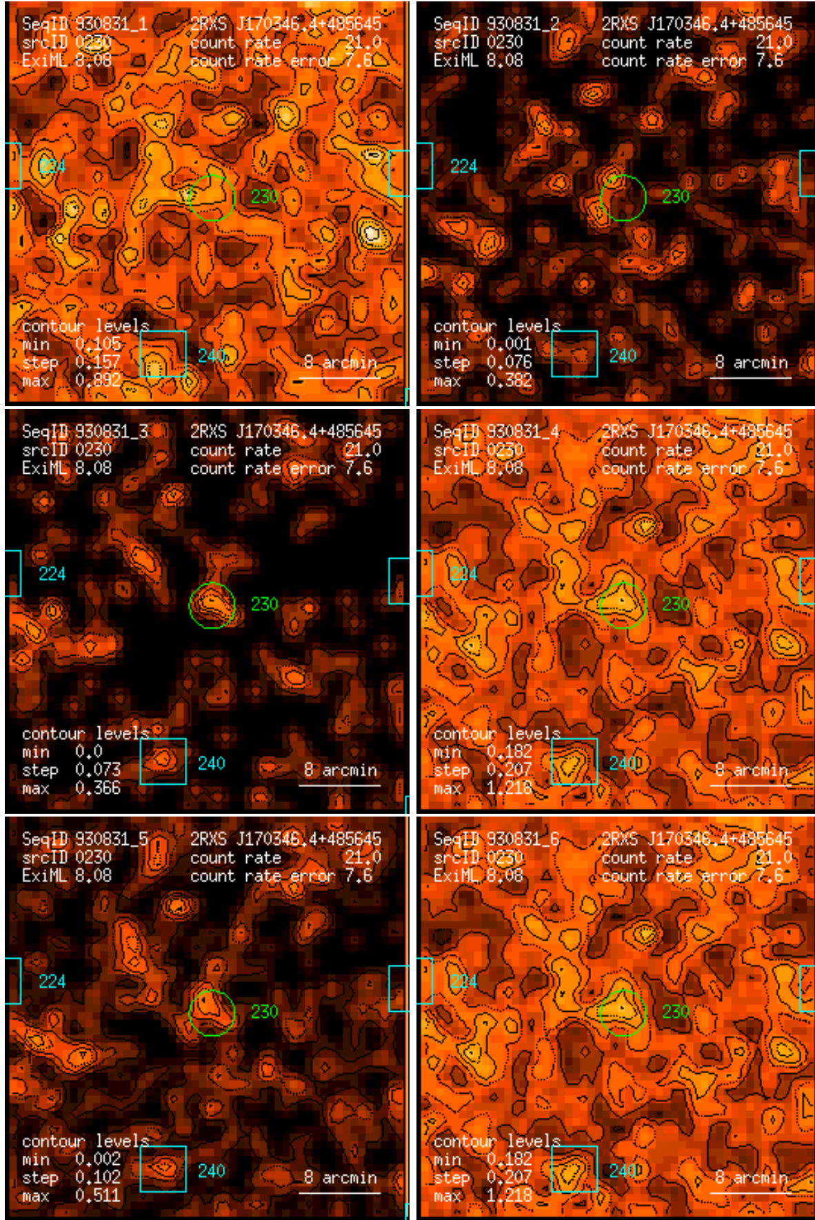
Figure 230: RASS 930831: detection 0230: band rate images, Gaussian filter: (1) PSPC channels 11 – 41, (2) 52 – 90, (3) 91 – 201, (4) 11 – 235, (5) 52 – 201, (6) 11 – 201. Broad band rates in counts/ks. Band rate contour levels in counts/ks/arcmin 2 .
